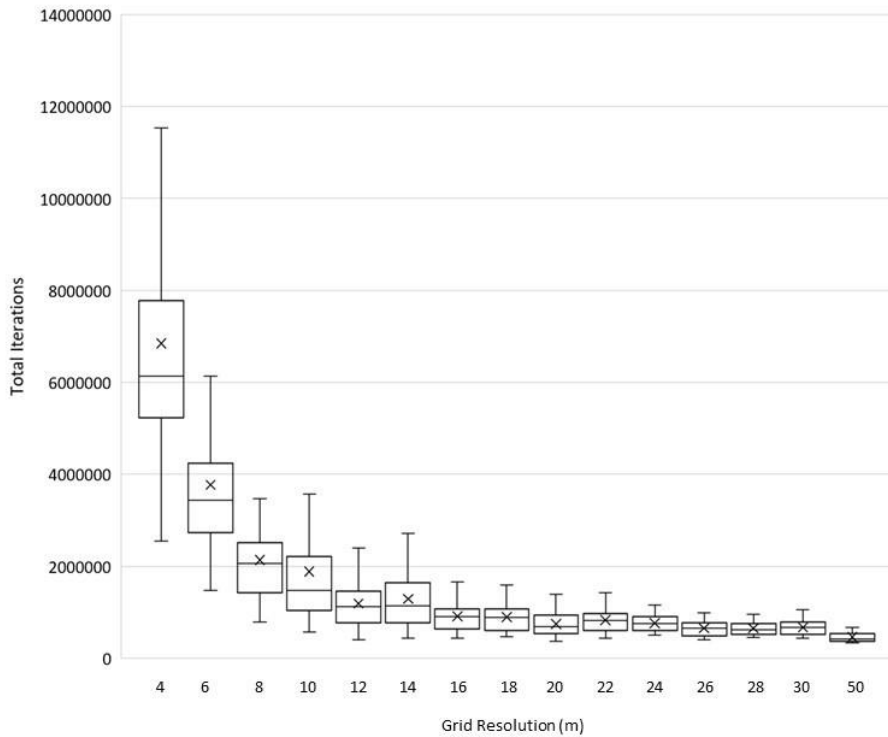
330 Figure 6 – Box-Whisker plots showing the spread of total number of model iterations required at each grid resolution.
