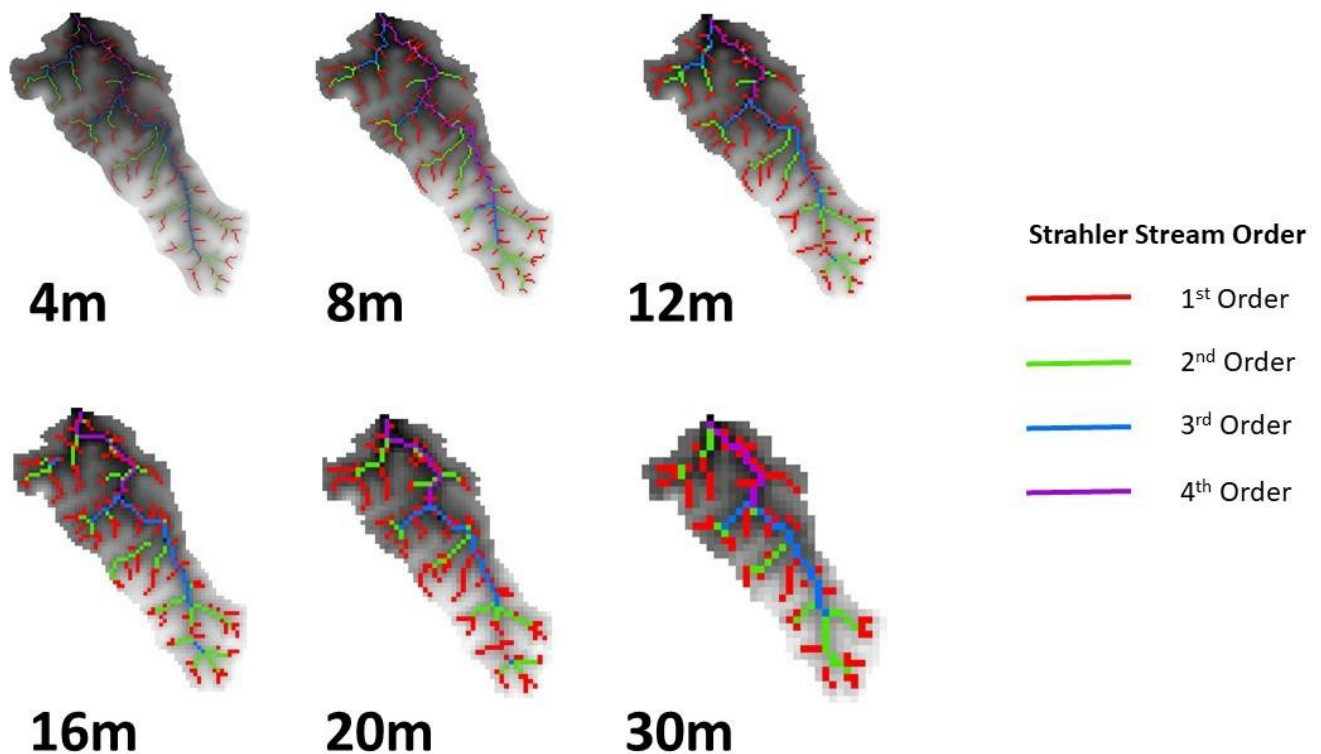
365 Figure 8 – Illustration of the loss of granularity in the representation of the stream network (shown is red) with increasingly large grid cell sizes.
