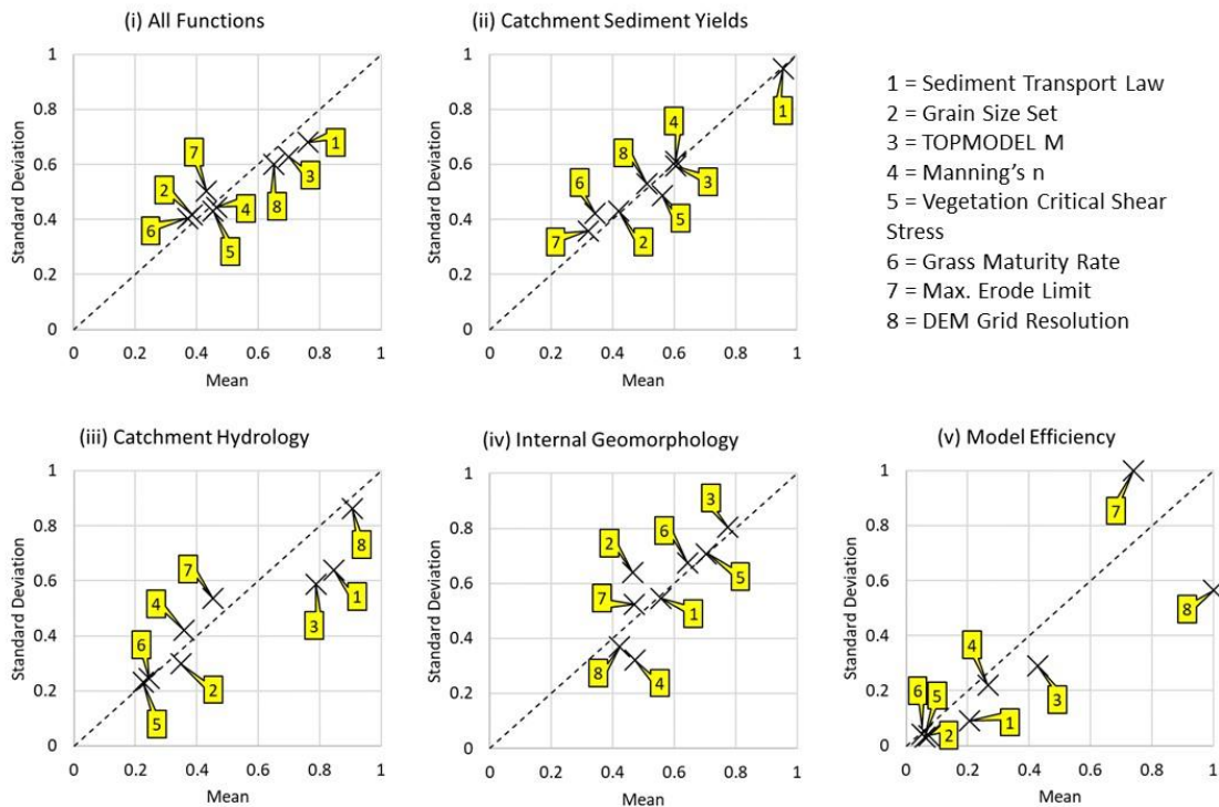
340 Figure 7 - Mean and Standard Deviation of relative MEs for the seven parameters and DEM Grid Resolution for all Model Functions aggregated by Core Behaviours (see Table 2).
