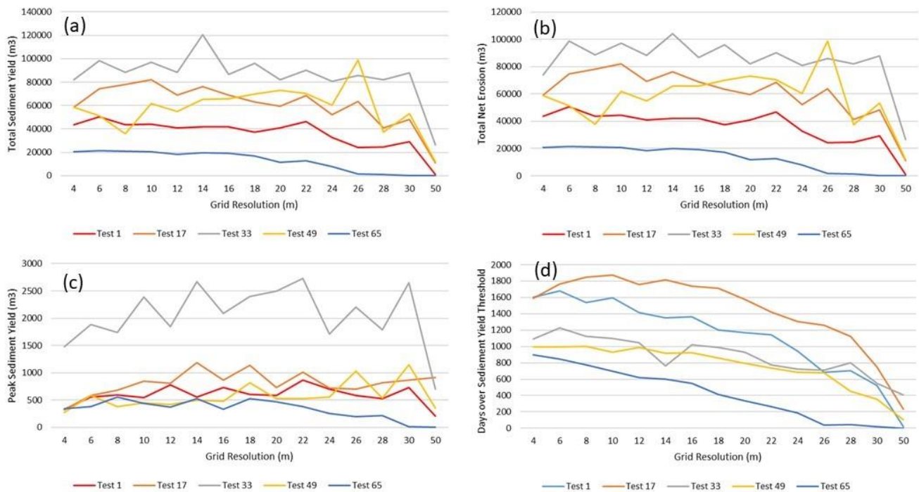
Figure 3 – Output values for five randomly selected test numbers at each grid resolution, for (a) Total Sediment Yield, (b) Total Net Erosion, (c) Peak Sediment Yield, and (d) Days over Sediment Yield Threshold.
