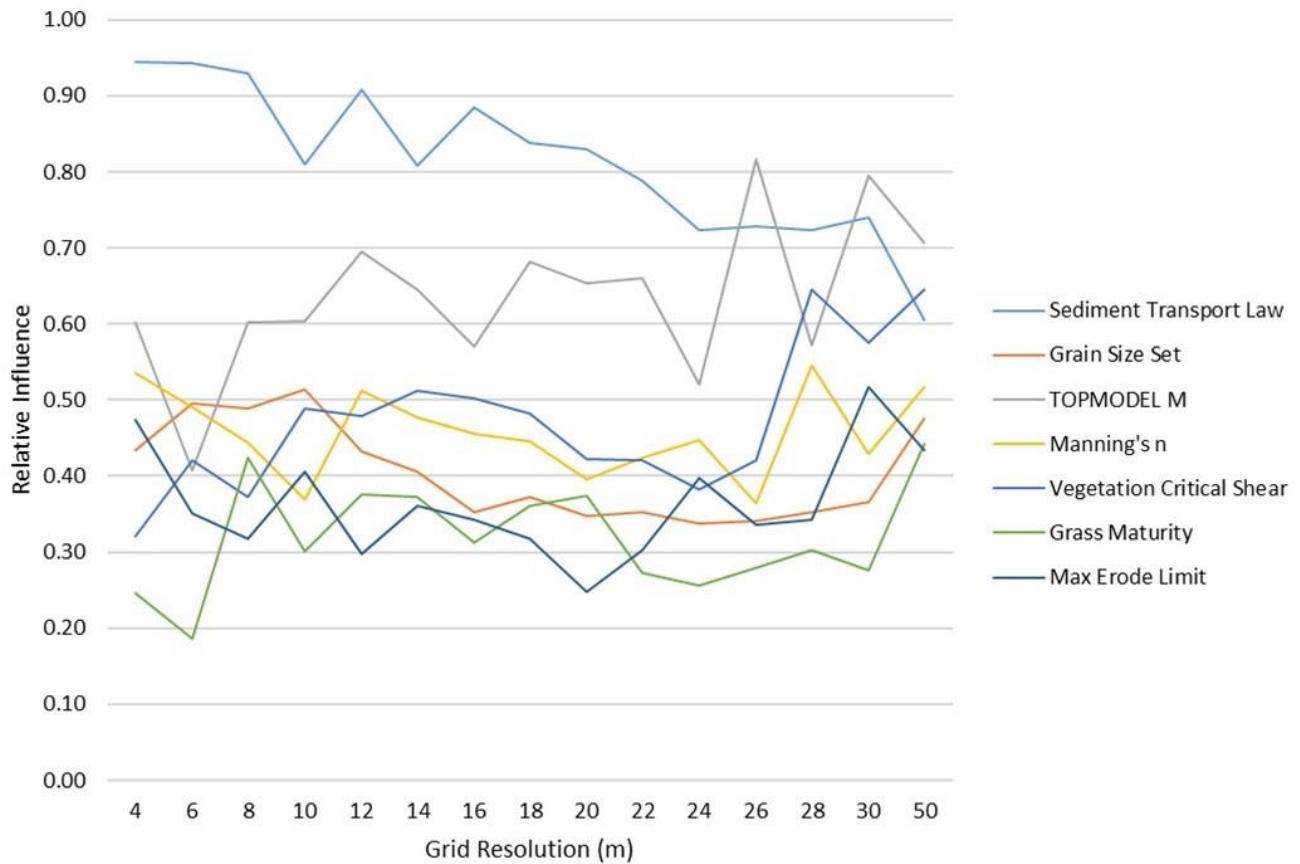
305 Figure 4 - Mean ME scores aggregated for all Model Functions for each parameter and each grid cell size.
