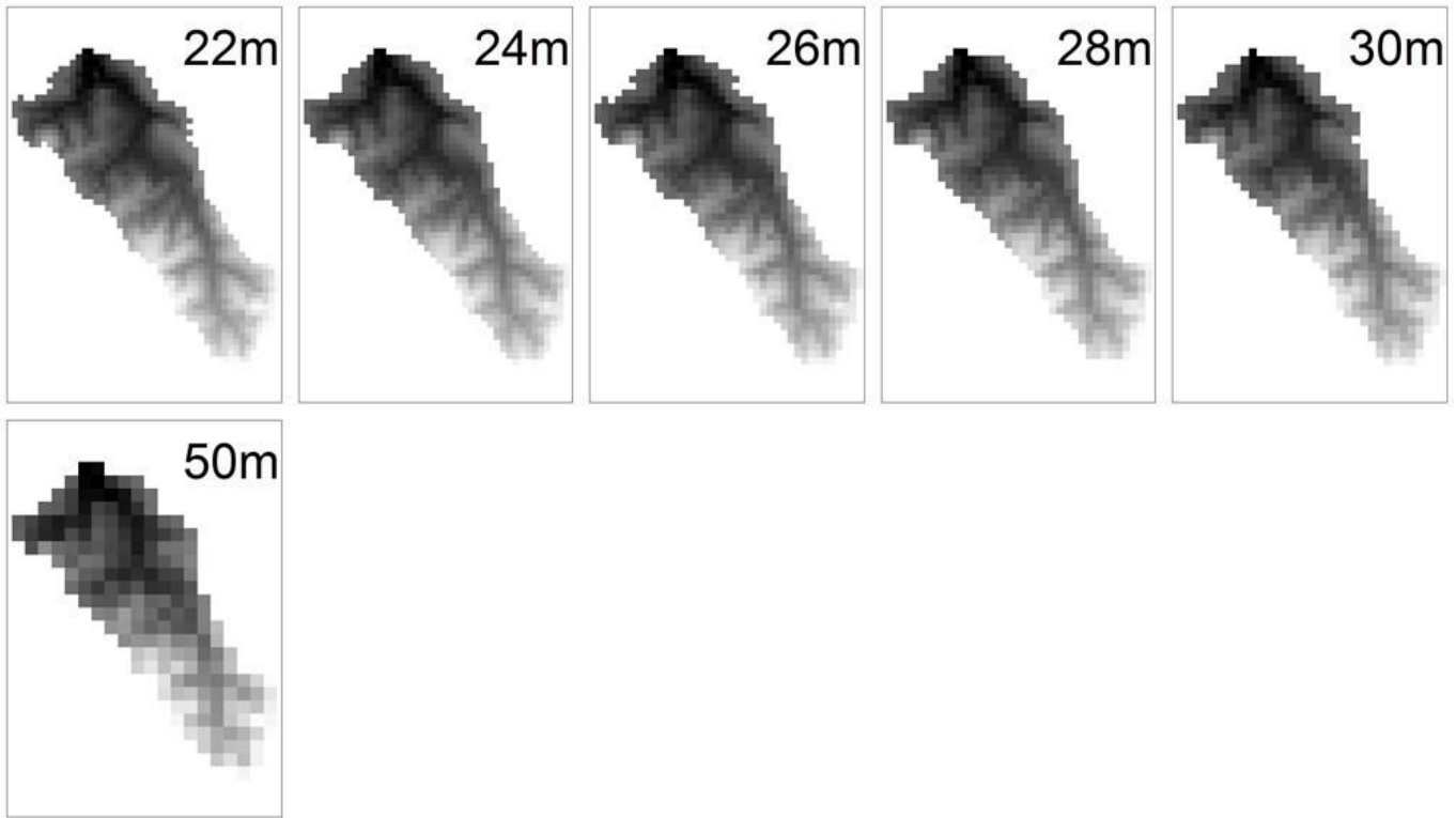
475 Figure A1 - Illustrations of the Tin Camp Creek DEM resampled at 2m increments, from 2m grid resolution to 30m, plus 50m.
