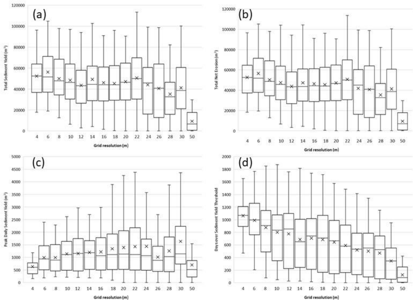
295 Figure 2 – Box and whisker plots showing the mean and spread of model outputs at each grid resolution, for (a) Total Sediment Yield, (b) Total Net Erosion, (c) Peak Daily Sediment Yield, and (d) Days over Sediment Yield Threshold.
