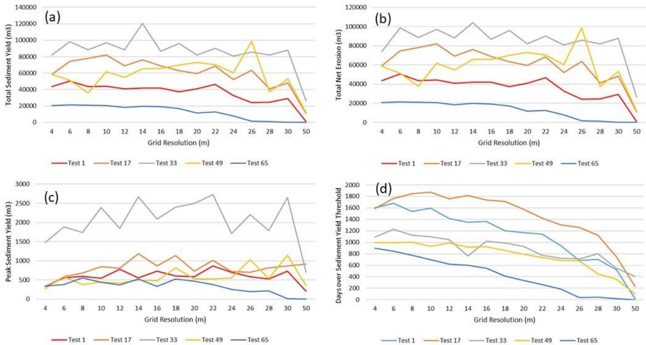
305 Figure 3 – Output values for five randomly selected test numbers at each grid resolution, for (a) Total Sediment Yield, (b) Total Net Erosion, (c) Peak Sediment Yield, and (d) Days over Sediment Yield Threshold.
