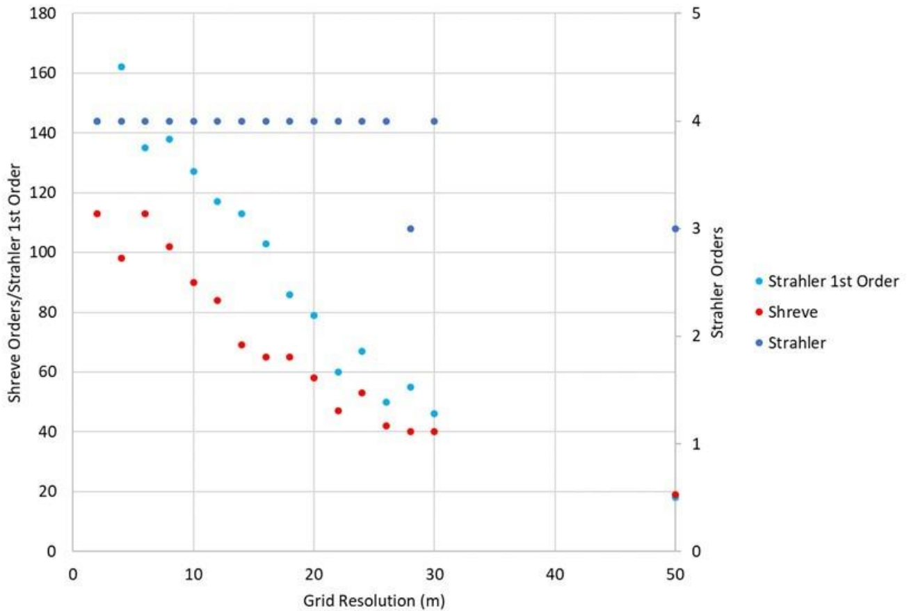
330 Figure 5 – The maximum number of stream orders calculated at each grid resolution using both the Strahler and Shreve methods. The total number of 1 st Order stream cells calculated by the Strahler method is also shown.
