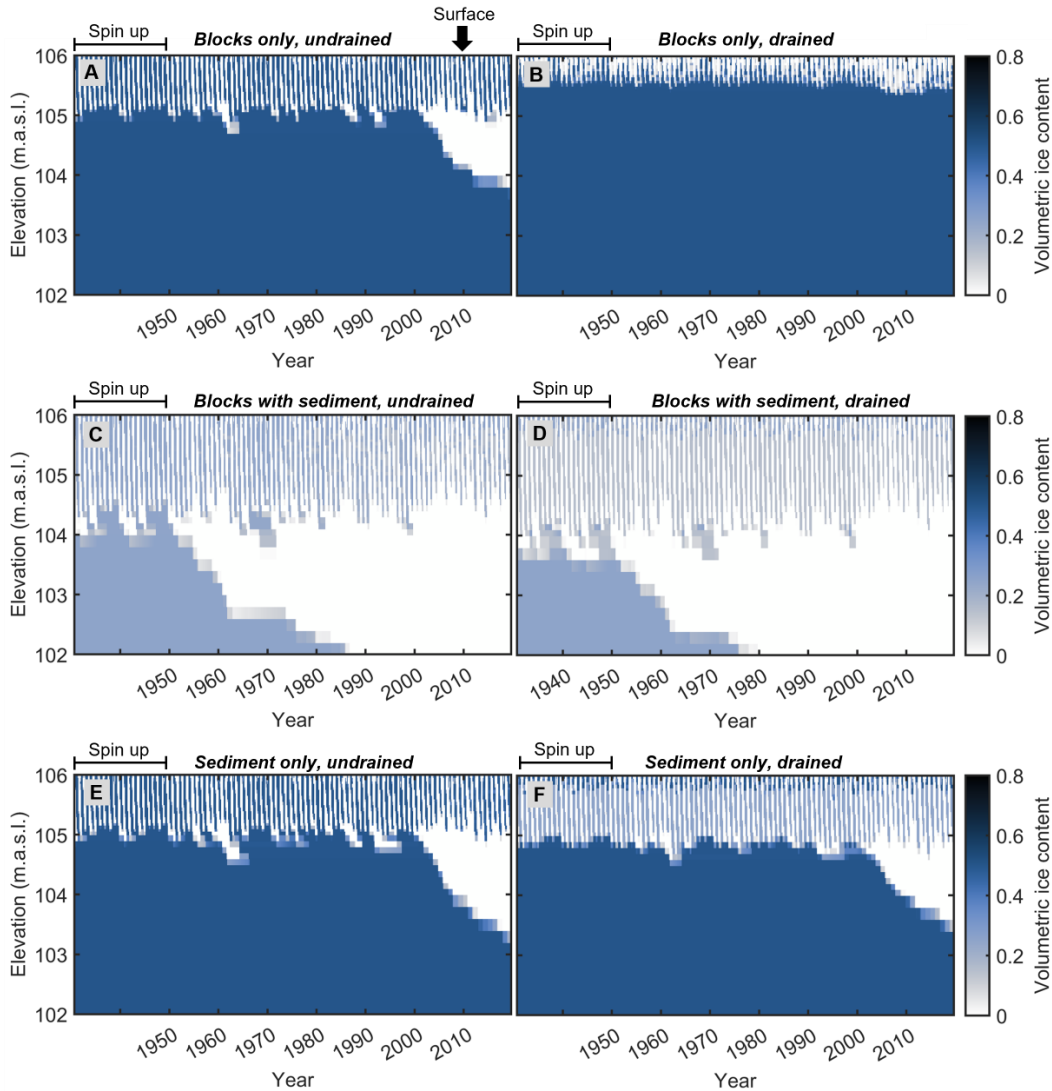
Line 420-423: Figure 8: Modelled volumetric ground ice content at Ivarsfjorden between 1951 and 2019 for the idealized stratigraphies in undrained and drained conditions and sf = 1 . The ground surface elevation is at 106 m.a.s.l. in the active layer, ice contents increase and decrease annually, corresponding to the active layer refreezing and thawing.
