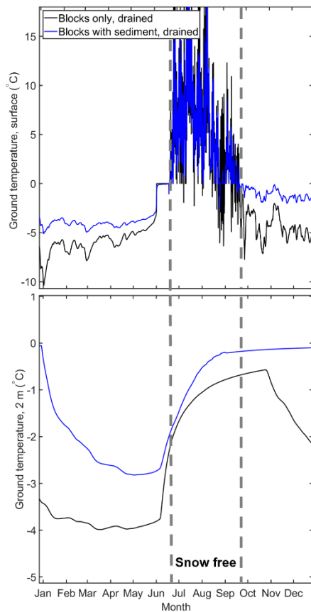
Line 385-388: Figure 6: Modelled ground temperature at 0.05 m (top) and 2 m (bottom) depth for the blocks only, drained and blocks with sediment, drained scenarios during a year of an equilibrium run at Juvvasshøe for sf = 0.75 . The snow-free summer season is highlighted. Note that the upper plot is truncated at 17 °C, maximum summer temperatures are 26 °C in both scenarios.
