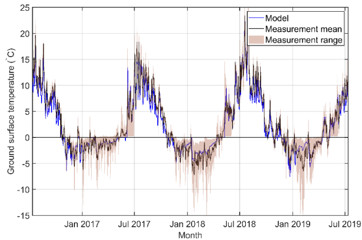
Line 349-352: Figure 4: Daily modelled and measured ground surface temperatures in Ivarsfjorden from July 2016 to July 2019. The shaded area indicates the minimum to maximum range of measured daily values from 11 loggers (based on Lilleøren et al., 2022), while the black line represents the mean value of all loggers.
