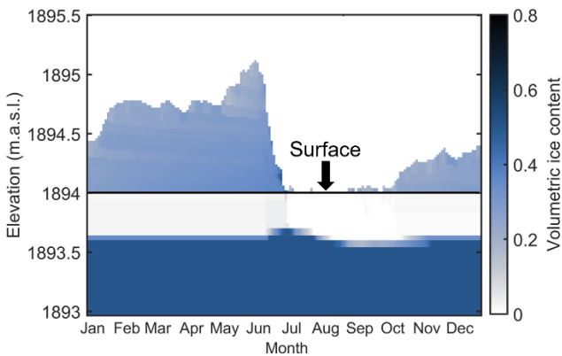
Line 397-400: Figure 7: Modelled volumetric ground ice content in the upper 1 m of the ground (below 1894 m) and the snow cover (above 1894 m) for the blocks only, drained scenario, during one year of an equilibrium run at Juvvasshøe for sf = 0.75 . Note the rise of the ground ice table in June after infiltrated snow melt water refreezes.
