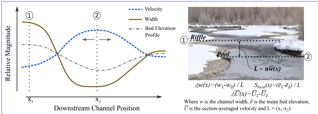
Figure 1. Conceptual diagram illustrating an inverse correlation between channel width and the section-average width-average flow velocity, or the local shear velocity, and the likely resulting bed topography profile. The inverse correlation has been shown to occur along river segments, and has been reproduced by numerical simulations of pool-riffle sequences as well as analogue physical experiments (Thompson et al., 1999; de Almeida and Rodríguez, 2012; Bolla Pittaluga et al., 2014; Nelson et al., 2015; Chartrand et al., 2018). The gray arrows indicate that the location of the velocity maxima (and minima) shift depending on the flow stage (Wilkinson et al., 2004). Photograph at right shows a gravel-bed river at spring rising snowmelt stage with a width change gradient from points 1 to 2 over a distance n\bar{w}(x) , where n can vary from 1 and higher. Bed architecture at point 1 is a riffle and at point 2 is a pool. Flow direction is from top to bottom of image. Note the broken water surface as flow transitions into the narrower location at point 2. Photograph by S.M. Chartrand, Flat Creek, near Jackson Hole, WY, U.S.A.
