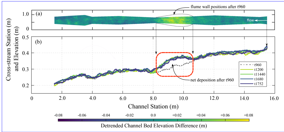
Figure 5. Bed elevation and profile changes after the width reduction was removed. (a) DEM of difference between t960 and t1200 min. The width profile for t960 used to show elevation differences because it was narrower within the central part of the flume compared to t1200 min. Width profile following t960 min shown with the light gray lines. (b) Trended mean channel bed profiles for t960, t1200, t1440, t1680 and t1752 min. Dashed red box lines up with region where the width reduction was removed following t960 min. Profiles calculated as width-averaged conditions with a resolution of 0.002 m.
