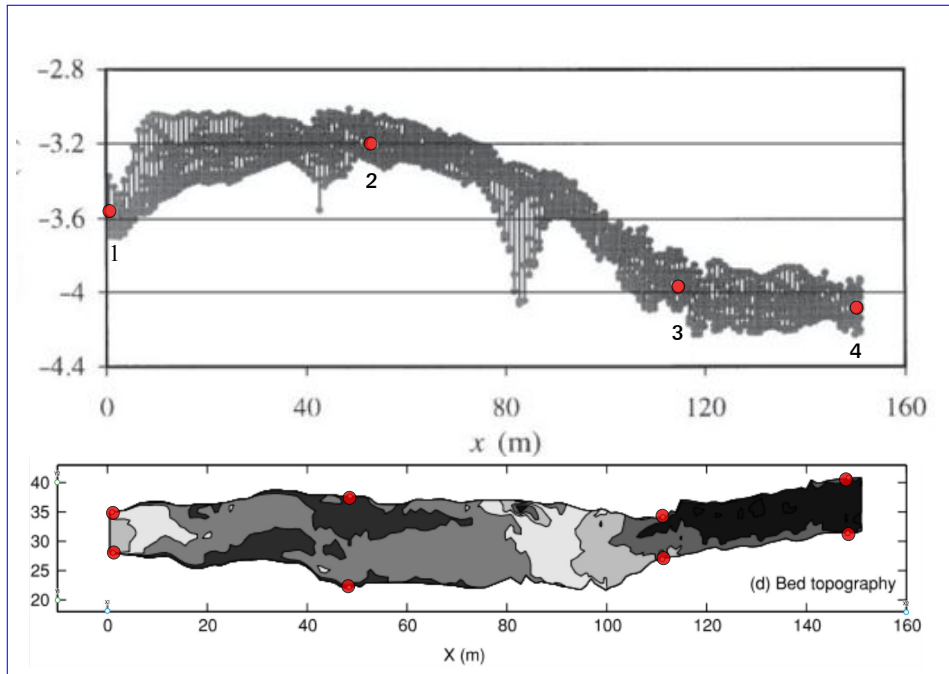
Figure B.3. Modified Figures 4 (top) and 3 (bottom) of Cao et al. (2003) showing the locations of channel width and elevation profile measurements indicated by the open circles. The bed elevation series is at the top of the image and the width series is at the bottom. Here channel width was measured as the distance in between the points at the two bounding edge positions at a given channel station. Units are meters. Flow is left to right in the image.
