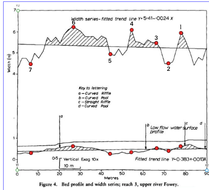
Figure B.2. Modified Figure-Fig. 4 of Richards (1976) showing the locations of channel width and elevation profile measurements indicated by the open circles. The width series is at the top of the image and the elevation profile series is at the bottom. Units are meters. Flow is right to left in the image.
