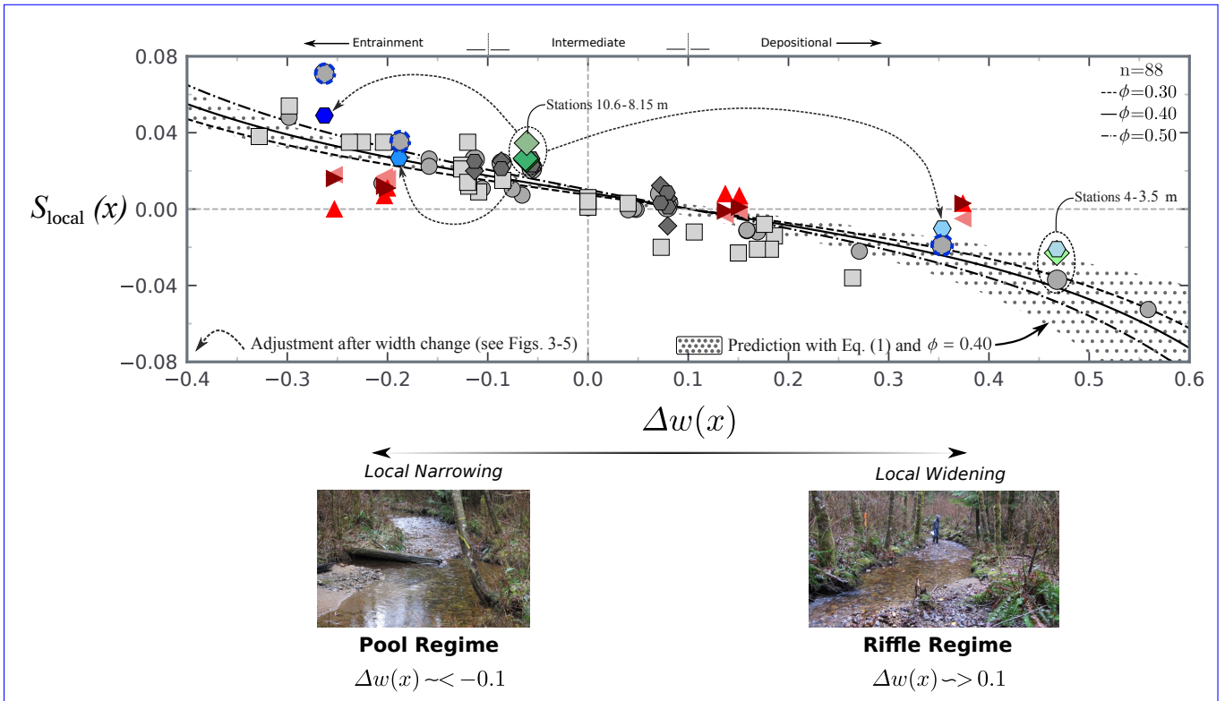
Figure 6. Local average bed slope S_{local}(x) as a function of the downstream channel width gradient \Delta w(x) for PRE4, and a wide range of additional field, numerical and experimental studies. Present experiment: \blacklozenge –Phase 1 PRE4, and \bullet –Phase 2 PRE4 at locations where channel width is adjusted during the experiment; \blacklozenge –Phase 1 PRE4, and \bullet –Phase 2 PRE4 at locations where width remains unchanged during the experiment; \bullet –Result from Chartrand et al. (2018) comparable to PRE4 for the same downstream width gradient. Literature-based data sets: \bullet –Chartrand et al. (2018) which includes data from Thompson et al. (1999) [field], de Almeida and Rodríguez (2012) [numerical], Bolla Pittaluga et al. (2014) [numerical] and Nelson et al. (2015) [experiment]; \square –Includes data from Richards (1976) [field], Cao et al. (2003) [numerical] and Vahidi et al. (2020) [experiment]; Red triangles include data from Brew et al. (2015) [field]; \blacktriangleleft –For the period before the Elwha and Glines Canyon Dams were removed on the Elwha River, \blacktriangle –Following removal of the Elwha Dam, and all but 30 feet of the Glines Canyon Dam, in the spring prior to the freshet floods, and \blacktriangleright –In the late summer after the freshet floods, and with the remaining 30 feet of Glines Canyon Dam still in place. See Appendix A for more details regarding the literature-based data sets \square . Plotted lines represent the centre of a distribution of predicted values using Eq. 1 for differing values of the packing fraction \varepsilon . See Appendix A and the online repository (Chartrand et al., 2022) for calculation procedure of Eq. 1. Distribution of predicted values shown with hatching for \phi=0.40 .
