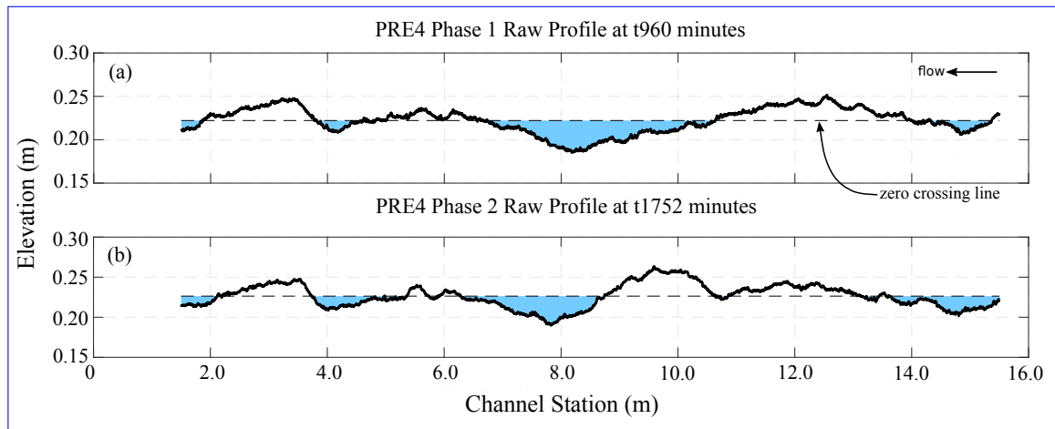
Figure 4. Detrended bed elevation profiles showing a zero-crossing line for Phases 1 and 2 of PRE4. (a) Bed elevation profile at t960 min, and (b) bed elevation profile at t1752 min, each calculated as width-averaged elevations at a resolution of 2 mm. Both profiles are fit with a zero-crossing line (Richards, 1976). The elevation profiles do not have a trend, and were sampled from the raw digital elevation models (see Chartrand et al. (2018) for more details regarding measurement methods for flume-bed elevations). Pool-like features are shown with blue shading below the zero-crossing line.
