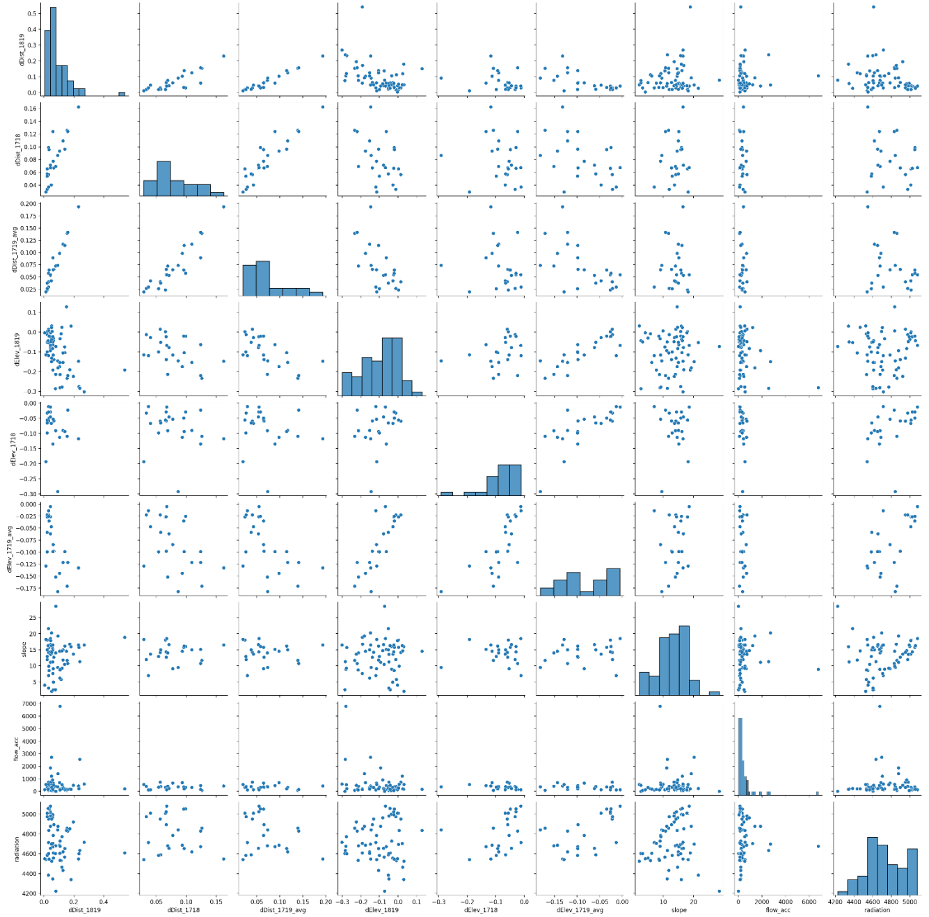
5 Figure S2: Pairplot of relationship between yearly vertical and horizontal DGPS-derived 6 displacements as well as terrain attributes as described in the text. “dElev” denotes change in 7 elevation, “dDist” denotes change in distance.
