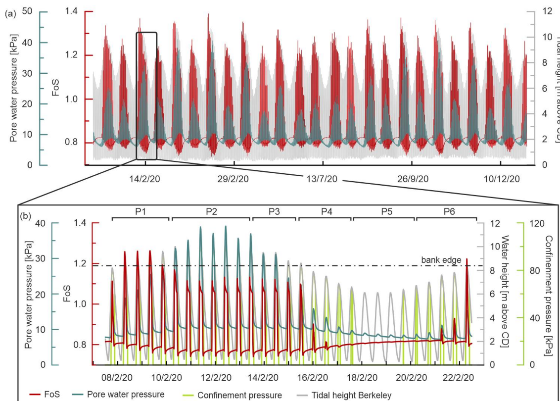
410 Figure 10. (a) Computed bank stability analysis for the year 2020 (b) Zoom into the period covered by the groundwater table monitoring in February 2020. This second plot is subdivided into different Phases (P1, P2, P3, etc) and pore water pressures are plotted for a representative cell the location of which is highlighted on Figure 6.
