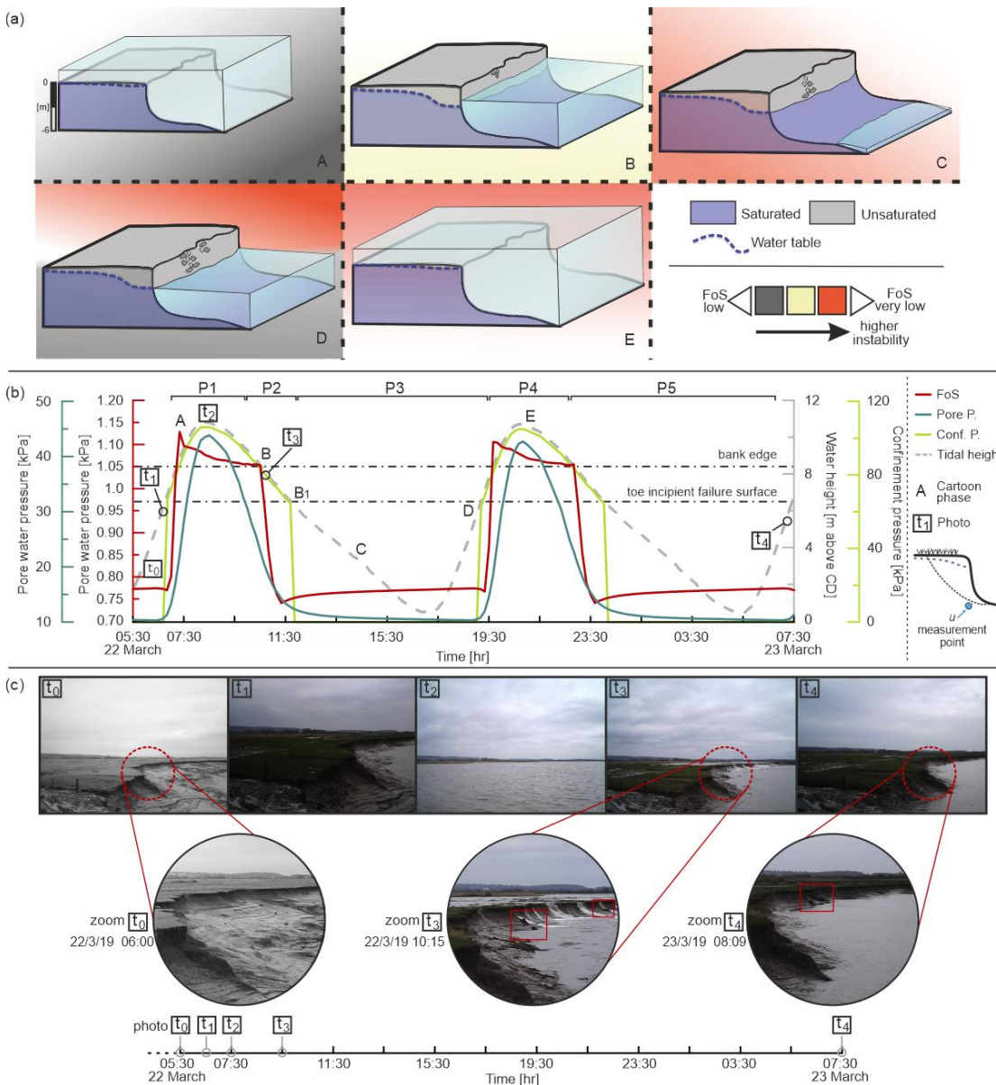
395 Figure 9. Simulated and observed (from fixed camera images) bank stability conditions at the Plusterwine study area during a 26 hrs time lapse (22-23 March 2019). (a) Cartoon of the studied bank and related conditions; (b) physical conditions of the bank. The letters refer to stages of evolution indicated on panel (a) and markers to photographs in panel (c).
