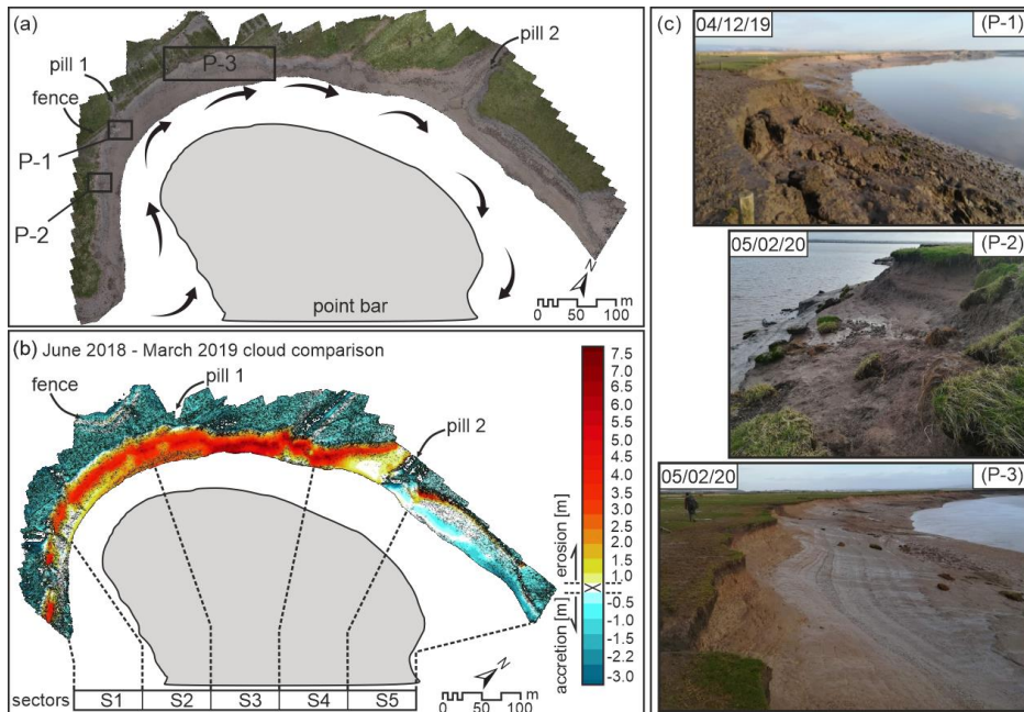
140 Figure 2. Embayment details (a) Studied embayment (mosaic of images), with inferred flood tidal flow represented by the black arrows; (b) point cloud difference between the June 2018 and March 2019 surveys and site subdivision into sectors, and (c) photographs of three representative areas of the study site shown in the black boxes on (a).
