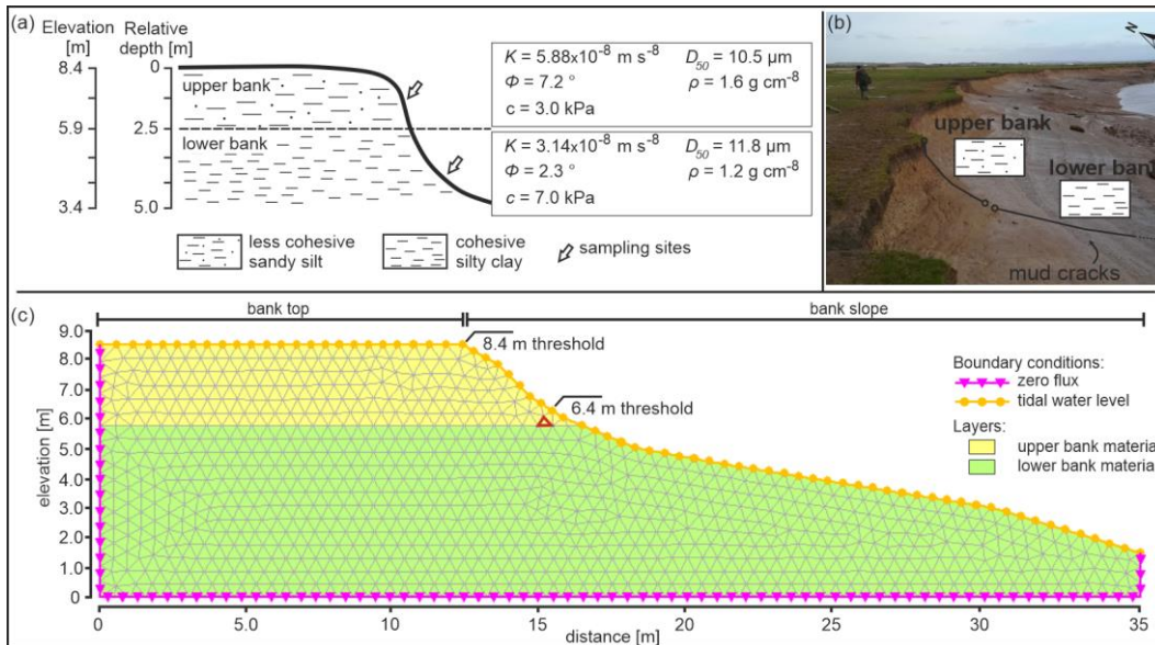
240 Figure 6. (a) Representation of the investigated bank at the study site illustrating the most important geotechnical characteristics of the two sedimentary layers ( K = conductivity, \Phi = angle of internal friction, c = cohesion, D_{50} = geotechnical grain size distribution, and \rho = dry bulk density). (b) Photograph of the central part of the study site showing the progressive change in grain size. (c) Representation of the mesh characteristics used in the bank stability model. The cell used to represent the temporal variations of the pore water pressure (see Figure 9 and 10) is highlighted in red. The different boundary conditions employed in the simulations are indicated. Note that the boundary condition indicated in yellow indicates the surface at which the tidal level interacts with the bank (with the entire bank slope in this specific example of high tide).
