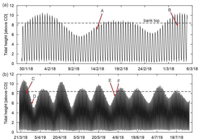
165 Figure 3. Tidal cycle for the two fixed camera survey periods: (a) 30/01/2018-05/03/2018; (b) 19/03/2019-28/07/2019 (data from UK Admiralty Total Tide software). Red arrows indicate the most substantial bank collapse events (A to F) identified during the monitoring periods (see Figure 4).
