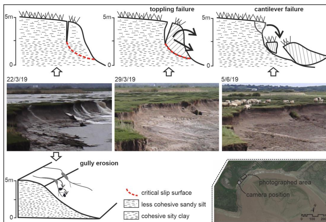
320 Figure 8. The typical collapse mechanisms observed at the study site (note that the photographs indicated refer to those presented in Figure 4). Image © Google Earth July 2021.
