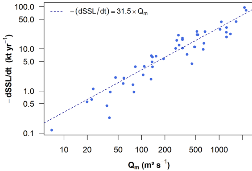
725 Figure 8: SSL-decline ( -\text{dSSL}/\text{dt} ) as a function of discharge for all stations with a significant change of SSL between 1990 and 2010. Linear regression
