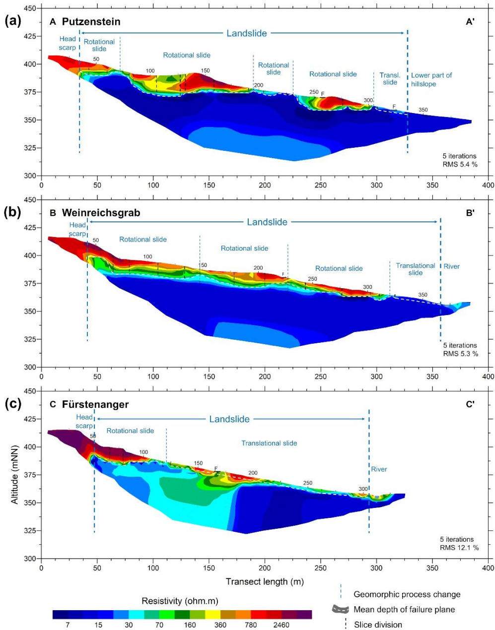
Figure 45: Geoelectric models and landslide forms at (a) Putzenstein, (b) Weinreichsgrab and (c) Fürstenanger. Failure plane depth was derived from vertical resistivity decrease in order of one to two magnitudes. For detailed derivation, see Figure S3 in the Supplementary Information. F highlights location of forest roads.
