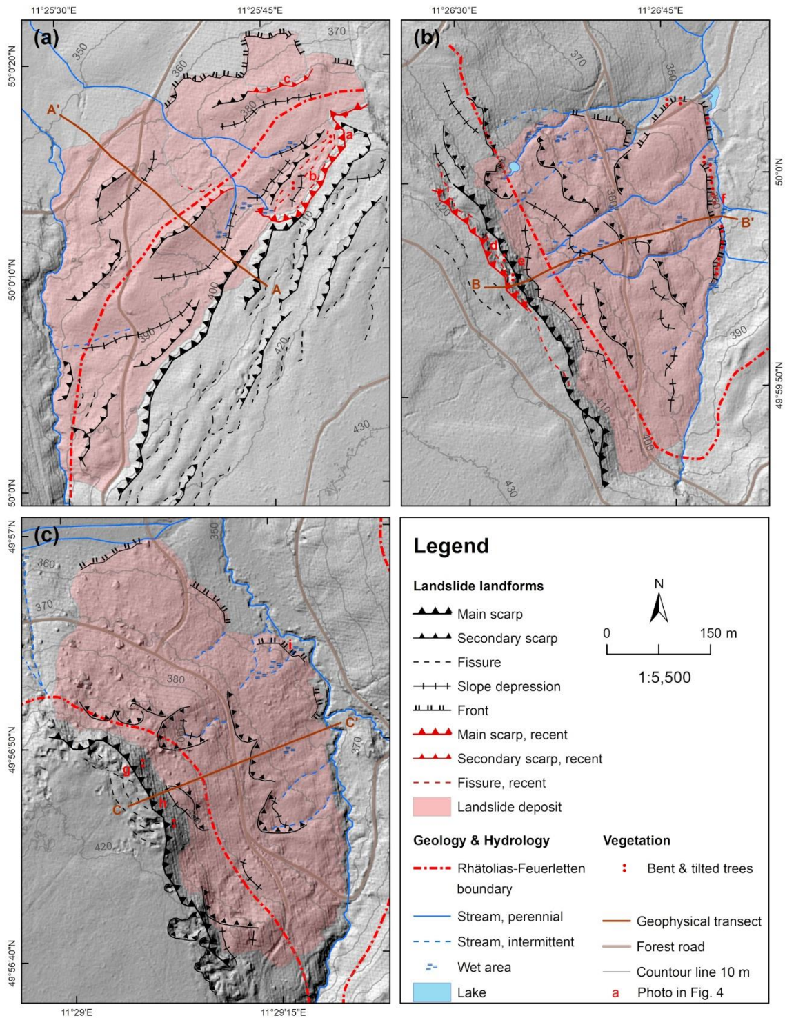
Figure 23: Geomorphic maps of the landslides at (a) Putzenstein, (b) Weinreichsgrab and (c) Fürstenanger (DEM source: Bayerische Vermessungsverwaltung). For location of landslides within the research area see Fig. 2b.
