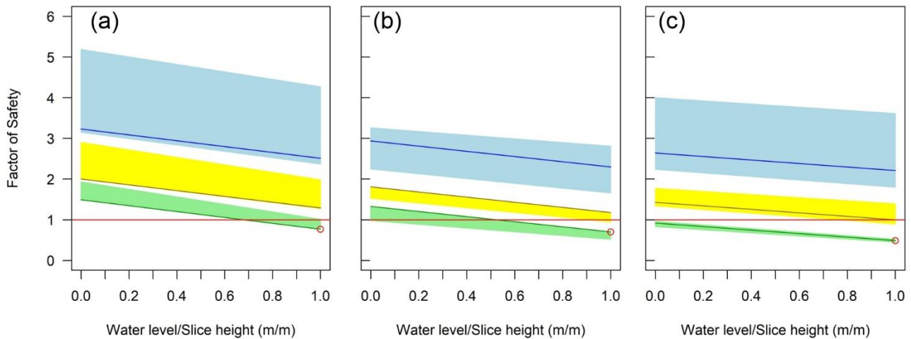
Figure 89: Factor of safety models for the reactivation of the landslides at (a) Putzenstein, (b) Weinreichsgrab, and (c) Fürstenanger. We assume an angle of internal friction of 8.4^\circ and \alpha^\circ . We vary cohesion between 28.6 kPa (blue scenario), 8.5 kPa (yellow) and 0 kPa (green). Calculations are based on a mean shear plane depth (line) and minimum and maximum shear plane depth (rectangle).
