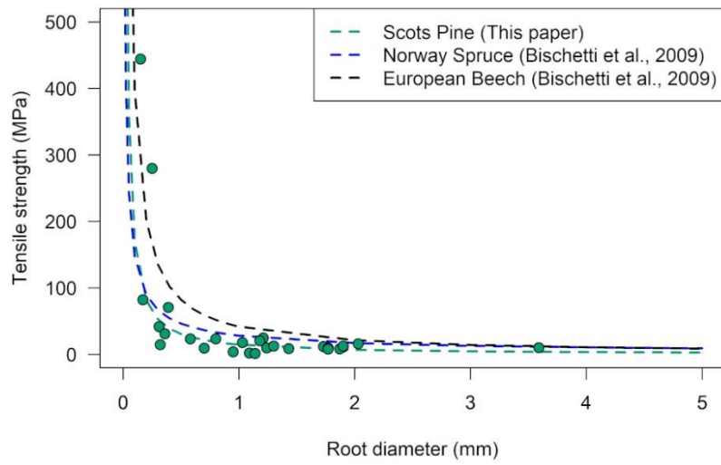
Figure 67: Tensile strength plotted versus root diameter for Scots pine compared to power laws derived for European beech and Norway spruce.
