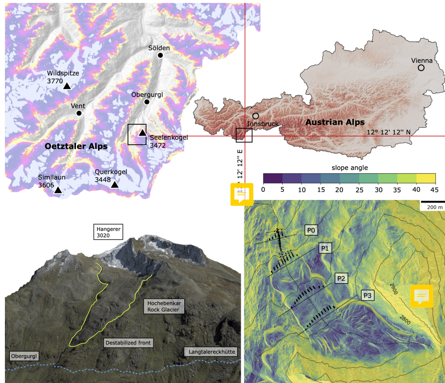
Fig. 1. Location of the study area in the Austrian Alps (top right) and detail of the geographical context of the Hochebenkar Rock Glacier in the Ötztal Alps (top left, the overlay shows the permafrost index map as per Boeckli et al. (2012); Boeckli et al. (2012)). Purple colour: Permafrost mostly in cold conditions). 3D visualization of the study site (data from SRTM and GoogleEarth, bottom left) and slope angle above hillshade generated from the 2017 DSM (bottom right). Black dots mark the positions of the blocks in the 4 cross profiles and the longitudinal profile for 2015-2021. Also shown are the central flowline and the lines between the fixed reference points that define the positions of the cross profiles.
