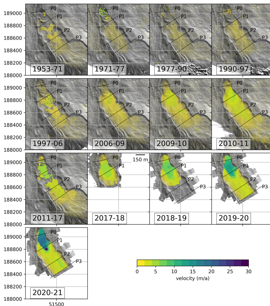
Figure 4. Velocity vectors (m/a) for the time series of DSM pairs, plotted over hillshades of the later DSM of each pair. Reference lines defining block profiles P0-P3 added for orientation. (Coordinate grid: EPSG: 31254)
