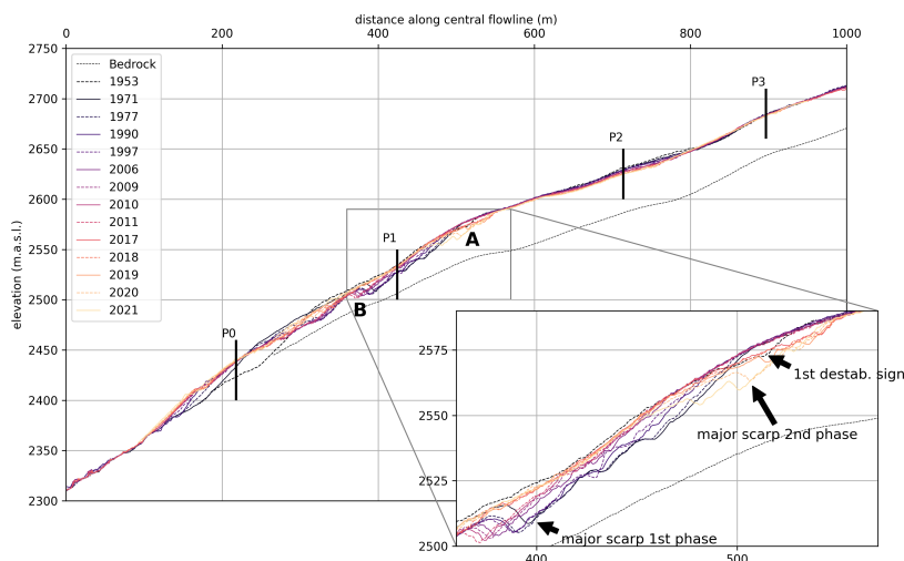
Figure 6. Surface elevation along the flow line as extracted from the DSMs. Estimated bedrock profile (dashed line) from Hartl et al. 2016b. Annotations show positions of the cross profiles. A and B mark upper and lower zones of morphological destabilization signs, as in Fig. 5.
