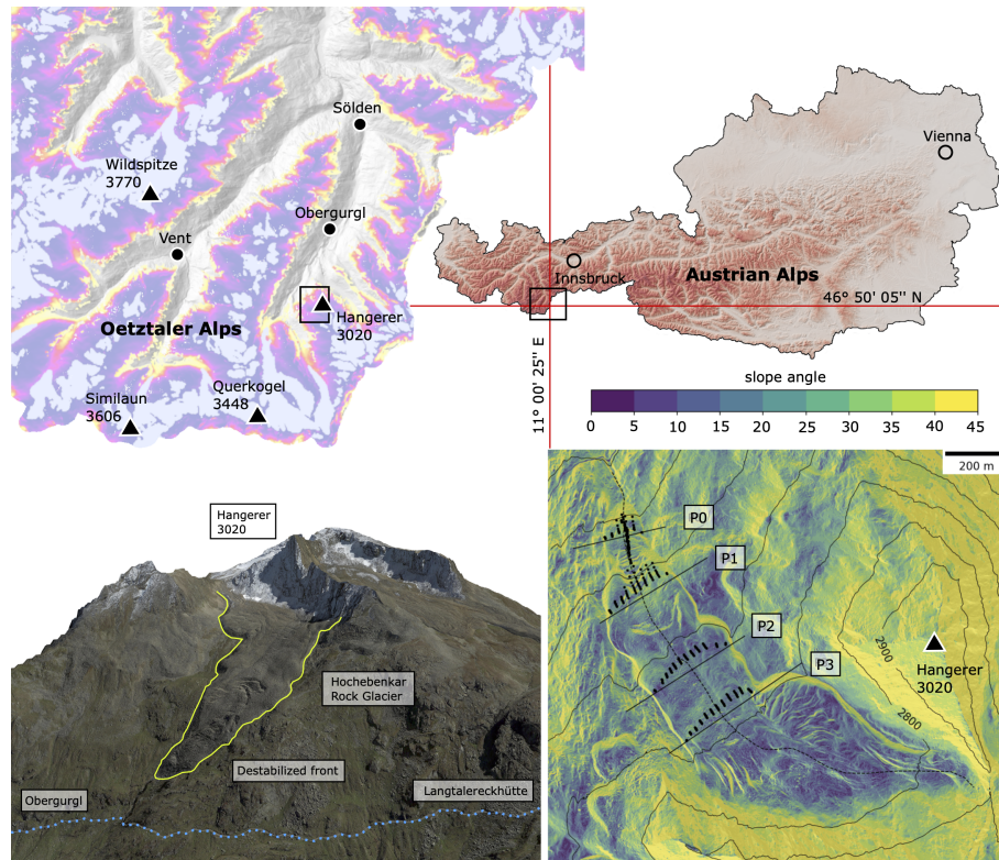
Figure 1. Location of the study area in the Austrian Alps (top right, base data: NASA Shuttle Radar Topography Mission (SRTM), red shading: elevation) and detail of the geographical context of the Hochebenkar Rock Glacier in the Ötztal Alps (top left, base data: SRTM, the overlay shows the permafrost index map as per Boeckli et al. (2012). Light blue color: Glacier; dark blue: Permafrost in nearly all conditions; purple: Permafrost mostly in cold conditions; yellow: Permafrost only in very favourable conditions). 3D visualization of the study site (data from SRTM and GoogleEarth, bottom left) and slope angle map draped over hillshade with contour lines, all generated from the 2017 DSM (bottom right). Black dots mark the positions of the blocks in the four cross profiles and the longitudinal profile for 2015-2021. Also shown are the central flowline (dashed black line) and the lines between the fixed reference points that define the positions of the cross profiles (solid black lines).
