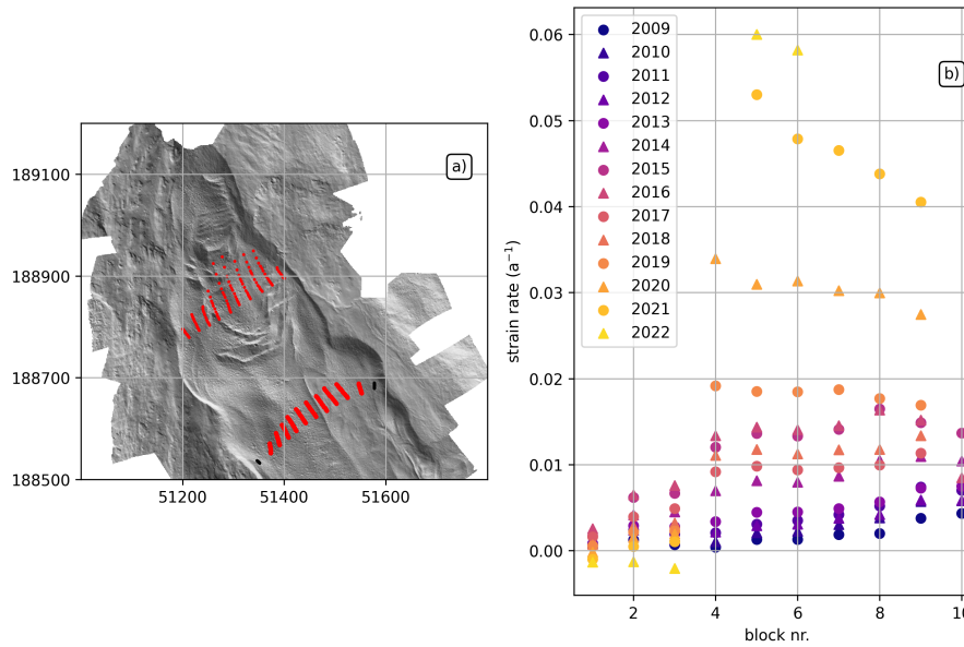
Figure 12. Strain rates for the blocks in P1 and P2 (excluding the furthest left and furthest right blocks in P2) for the measurement years 2009/10 to 2021/22. Panel a) shows the location of the blocks in each year (red dots) over the 2021 hillshade. Panel b) shows the strain rate per block pair, counting the blocks in the profile lines from west to east.
