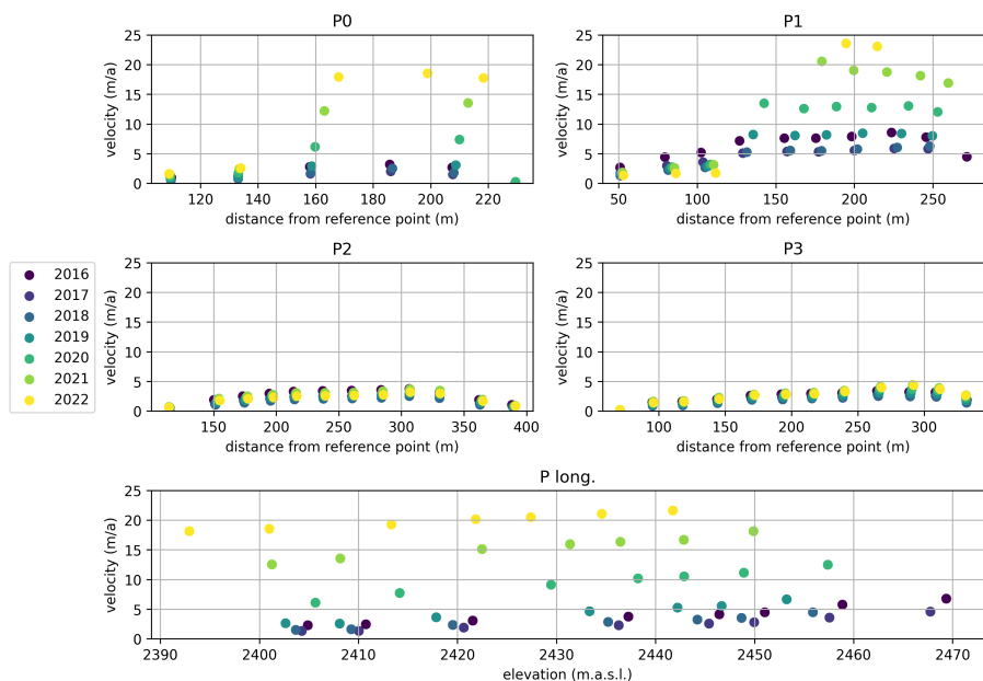
Figure 11. Block velocities for the four cross profiles (P0-P3) and for the longitudinal profile (P long.) in m/a for 2015/16 - 2021/22. The x-axis shows the distance from the orographic left reference point for P0, 1, 2, and 3, respectively. For P long., the x-axis shows the elevation of the blocks in each year. In P0, the third block from the right could not be located in 2018-2021, presumably because it rotated so that the marking was obscured. In P1, a block was similarly lost in 2021, and 3 more were lost in 2022. For P. long., only blocks that were found every year since 2016 are shown.
