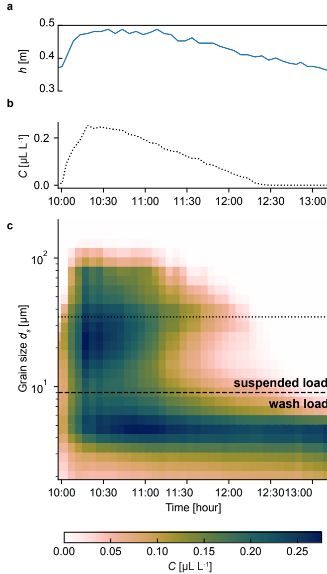
Figure 6. Data acquired with a LISST-Streamside in the Capesterre river, on October 30th 2011 2010 . (a) water level and (b) concentration of particles of median size 34.8 \mu\text{m} (class sizes between 31.9 and 37.7 \mu\text{m} ) as a function of time. (c) Evolution of the concentration (color code) as a function of time (horizontal axis) for each of the 32 classes of grain sizes (vertical axis). Dashed line : transition between wash and suspended load. Dotted line : concentration profile displayed in (b).
