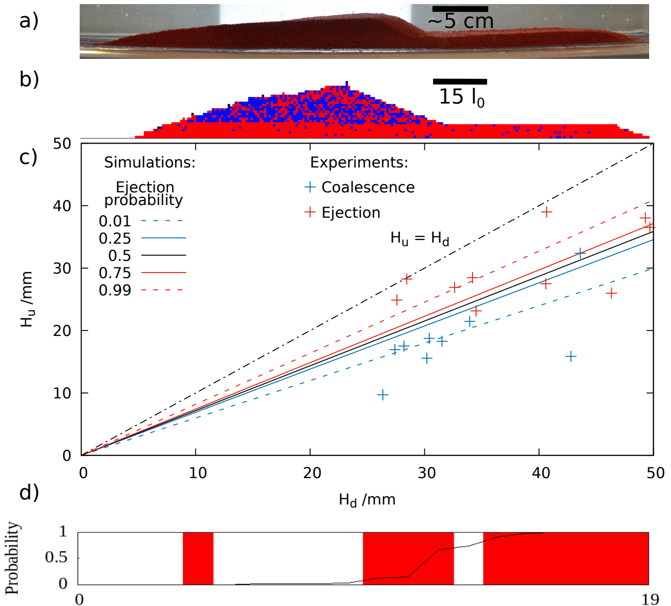
Figure 4. The morphology of intermediate bedforms in a) experiments of Jarvis et al. (2022) and b) simulations. Both show the distinctive plateau. c) The location of experimental ejection and coalescence events on the numerically-determined regime diagram. Most interactions result in their most likely outcome, with just four having a probability less than 0.5. d) A separation plot, generated by ordering the 19 experimental data points from panel (c) from smallest H_u/H_d on the left to the largest on the right. Instances resulting in ejection are represented as red columns. Overlain is a line chart showing the probability of each interaction resulting in ejection, as given by equation 5.
