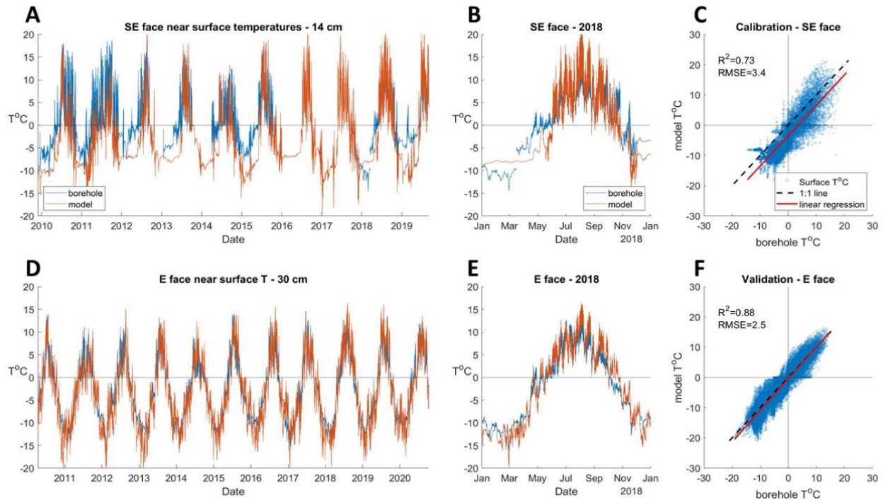
240 Figure 3: Comparison of near-surface temperature (T) data from model output and borehole measurements - A) Comparison of modeled near-surface temperature (orange) at depth 0.14 m, with borehole measurement from the SE face study site (blue). B) Same as A showing modeled and observed rock temperatures during the year 2018. C) Correlation of modeled near-surface temperature (depth=0.14 m) and borehole temperature, SE face, after calibration of snowfall multiplication factor (0.25) and
