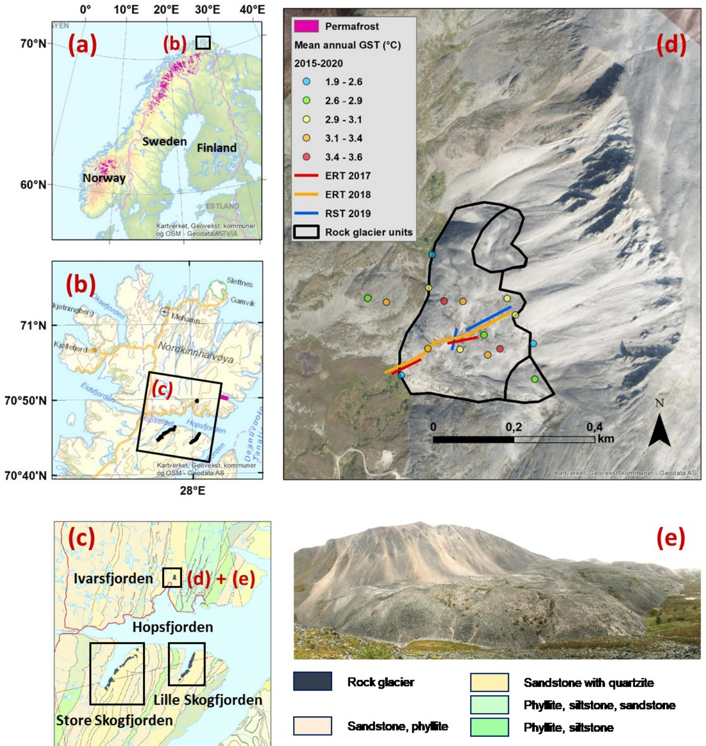
Figure 1: A: Overview map of Norway, Sweden and Finland (© ESRI and OpenStreetMap contributors), with our study area indicated by the black square B. Probable permafrost presence as modelled in Gisnäs et al. (2017) is shown in pink. B: Closer view
