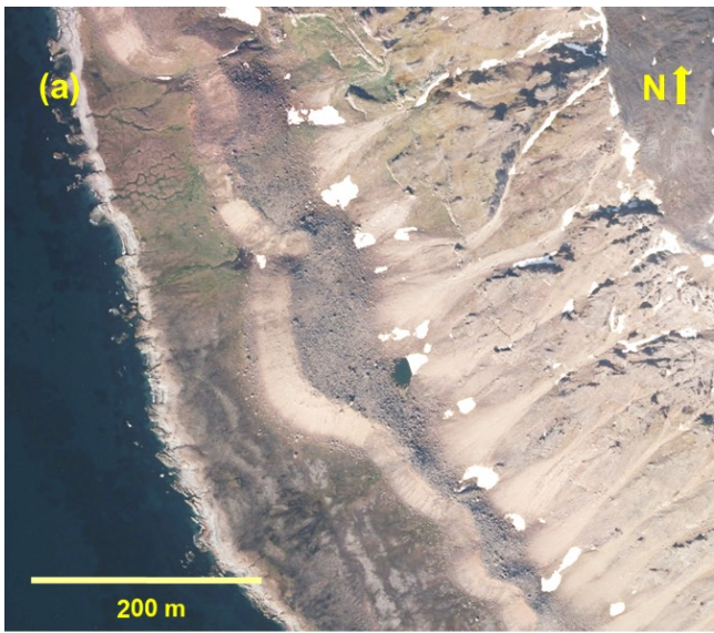
Figure 9: Comparison of landforms in (a) Svalbard (Prins Karls Forland; Western Spitsbergen; © Norwegian Polar Institute) and (b) Lille Skogfjorden, Finnmark (© Norwegian Mapping Authorities). In both cases the rock glaciers creep from talus slopes onto the strandflat. Especially in (b) the relict shorelines are visible.
