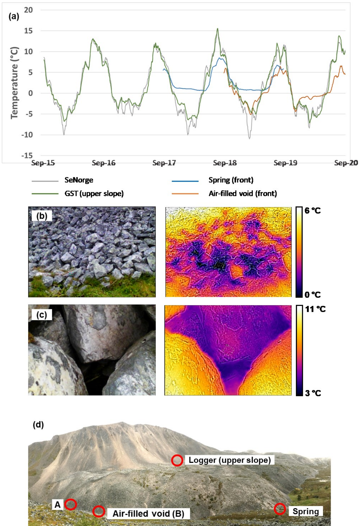
Figure 8: (a): Air and ground surface temperature over the 5 years of monitoring. The graph shows daily temperatures smoothed over 20 days; grey: SeNorge air temperature; green: ground surface temperature (GST) close to the top of the rock glacier; blue: temperature of water from spring escaping from the rock glacier front; orange: open blocks in the rock glacier front (positions indicated in image (d)). Images (b) and (c) show optical (left) and thermal (right) image of the rock glacier front. Positions can be found in image (d). Image (b) is also the location of the temperature measurements in orange above. Both images (b) and (c) are taken on 10th Sept. 2018. This day had air temperatures above 20 °C.
