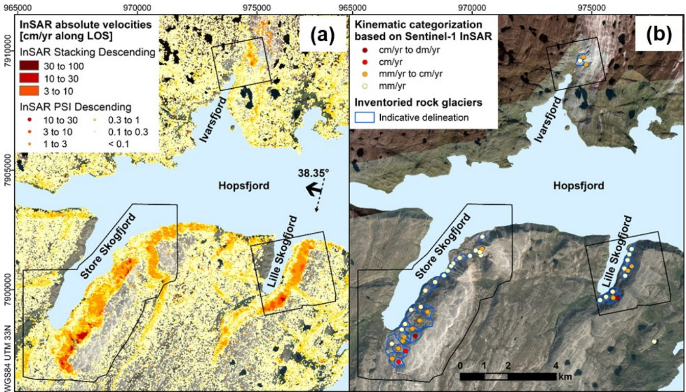
760 Figure 4: (a) Composite InSAR map based on classified mean annual ground surface velocities from snow-free Sentinel-1 satellite 765 images (June-October) between 2015 and 2020 (descending geometry). The map combines results processed with InSAR Stacking method (Rouyet et al., 2021) and Persistent Scatterers Interferometry (PSI) (NGU, 2020; Dehls et al. 2019), two methods that have complementary detection capabilities and therefore cover different velocity ranges. The black polygons show the extents of the geomorphological maps from fig. 2. The black arrow shows the direction of the flying satellite (dashed line) and the corresponding radar line-of-sight (LOS) towards WNW. The label above the LOS arrow indicates the angle between the vertical and the LOS. (b) Indicative delineation of rock glacier units and associated kinematic attribute (order of magnitude of the creep rate) based on Sentinel-1 InSAR velocity from (b). The background imagery are from “Norge i bilder” © Norwegian Mapping Authority, Projects: Nordkinnhalvøya 2012, Gamvik Lebesby Tana 2016, and Finnmark 2018. Retrieved from https://www.norgebilder.no/
