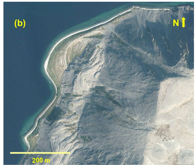
Figure 9: Comparison of landforms in (a) Svalbard (Prins Karls Forland; Western Spitsbergen; © Norwegian Polar Institute) and (b) Lille Skogfjorden, Finnmark (© Norwegian Mapping Authorities). In both cases the rock glaciers creep from talus slopes onto the strandflat. Especially in (b) the relict shorelines are visible.
