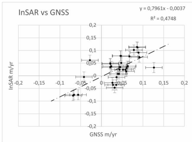
310 311 Figure 6. InSAR VS GNSS (LOS) data (m/yr). InSAR is not sensitive to velocities higher than 2 cm/yr. Therefore, we 312 mask all values that are related to GNSS values higher than |2| cm per year.
