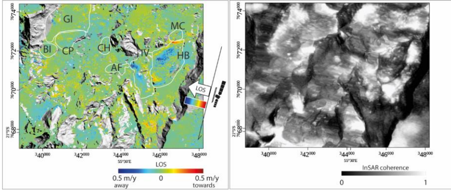
239 240 Figure 2. Left: InSAR velocity map in the LOS of the satellite, using the descending mode. A ground displacement 241 pattern is clearly visible in the Hell-Bourg area. Right: InSAR signal coherence. Coherence values lower than 0.3 are 242 masked in the left panel.
