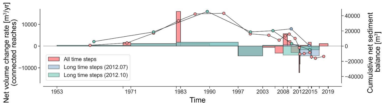
575 Figure 11: Net volume change rate (bar plot) and cumulative net sediment balance (dots) for the active floodplain for all time steps including monthly data (19 DEMs) and for longer time intervals (7 time steps, with a minimum interval of 4 years). For these time steps, we show the difference in the cumulative net sediment balance when the interval is between 2008-2012 July (before the heavy rainfall event) and between 2008-2012 October (after the heavy rainfall event).
