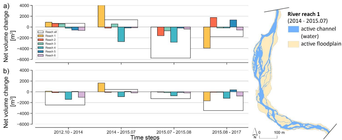
430 Figure 9: Net sediment volume change of the active floodplain for each reach and all connected reaches a) with and b) without considering the water surface in the calculation. On the right, the active floodplain and the active channel (i.e. the water surface, which area covers about 41 % of the active floodplain) is illustrated for reach 1. The mapping of the active floodplain and active channel for the other river reaches is shown in Figure S5 for the time step 2014-2015 July.
