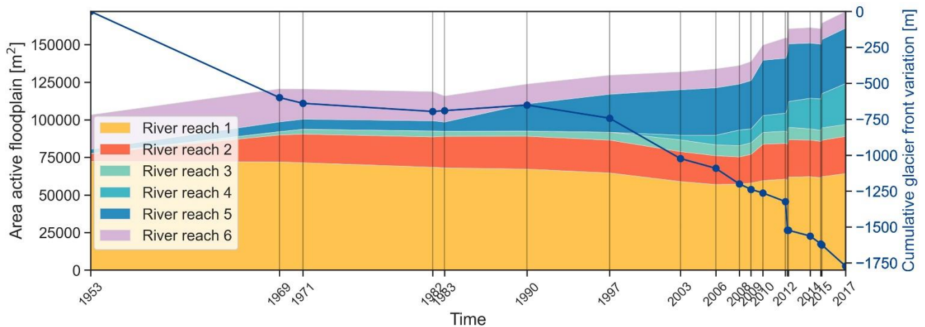
290 Figure 4: Area change in square metres of the mapped active floodplain and the cumulative glacier front variation. This is calculated with respect to the river centreline as of 2017. Note that the year 2019 surveyed by UAV is missing as there is no data up to the glacier front.
