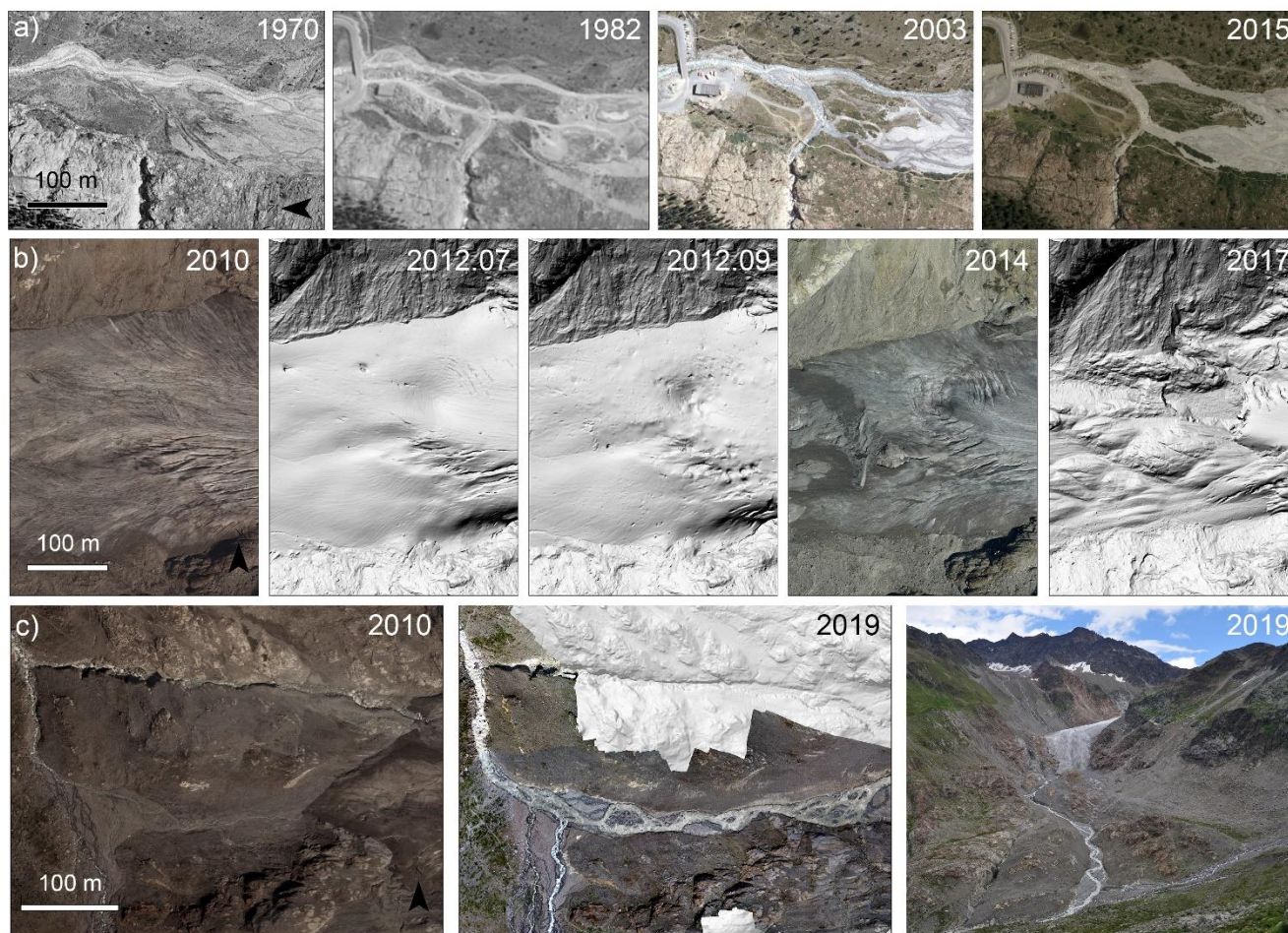
555 Figure 10: Orthophotos and hillshade DEMs of selected time steps that visually show a) the human activities on the river reach 1 downstream after 1970; b) the development of a circular pattern (2012 July) on the glacier and the outburst of subglacial water pocket and c) the proglacial area change over 9 years such as channel incision and rocky characteristics of the river bed.
