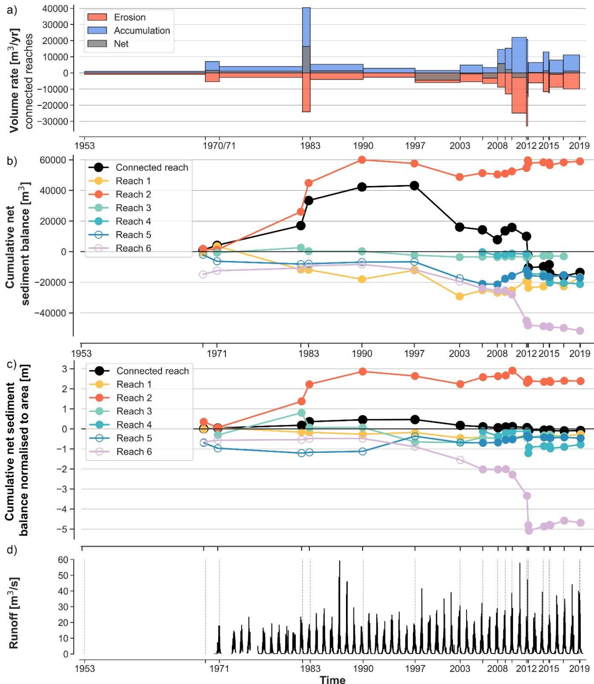
Figure 6: a) The volume change rate and b) the cumulative net sediment balance in cubic metres and c) in metres (i.e. normalised to area) for the connected reaches and for each river reach. Note that following the topology of the reaches and the time of their deglaciation, the net balance for the first time step contains reaches 1 and 2 only, reach 3 is included from the second time step onward, and reaches 4, 5, and 6 are contained in the balance from 2003 onward. The cumulative balance for the reach 5 and 6 is
