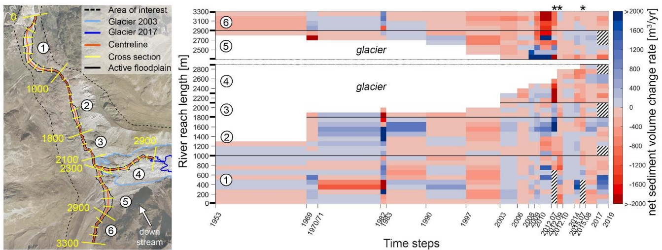
Figure 5: Spatio-temporal variation of the net sediment volume change rate of the active floodplain (reach 1 to 6) in cubic metres per year ( \text{m}^3/\text{yr} ). On the left, a graphic illustration of the length of the reaches and the cross-sections drawn every 100 m along the thalweg superimposed on the generated orthoimage of 2003. The arrow indicates the downstream direction. Negative values (reddish colours) represent surface erosion while positive values (blueish colours) represent surface deposition. For better visualisation, a limit of 2000 \text{ m}^3 per year is chosen. Missing information is indicated with a hatched area. Note that for the monthly time step, indicated with * in the figure, the absolute volume change (i.e. \text{m}^3 ) is reported instead of the volume rate. In addition, for better visualisation, their width corresponds to one year.
