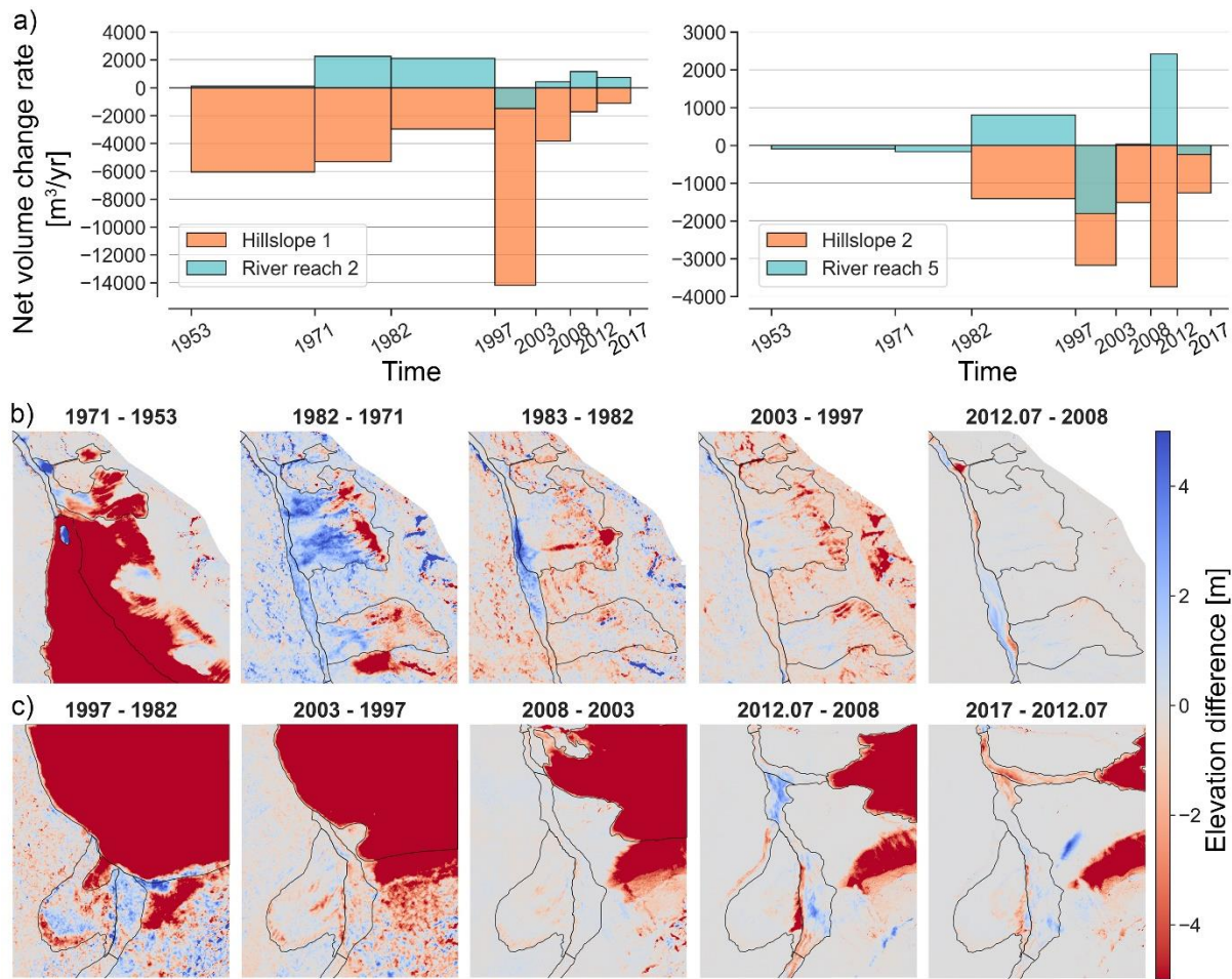
Figure 7: a) The rate of net volume change of lateral hillslope 1 and 2 (reference to Fig. 2) for the selected time steps and the corresponding net volume change rate of the active floodplain of the river reach 2 and 5, respectively. Note that sediment from hillslope 2 is transferred to reach 5 from 1982 onwards. For the selected time steps, the elevation difference map b) of the lateral hillslope 1 and c) the later hillslope 2, with the mapped active floodplain and glacier.
