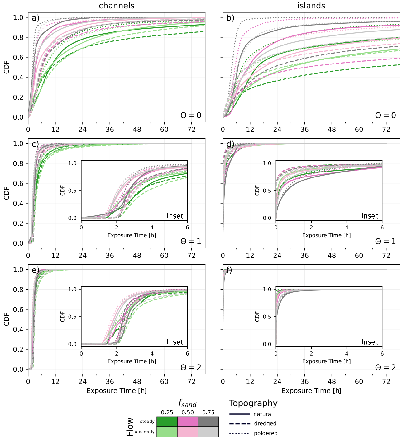
Figure 10. Exposure time cumulative distribution functions (CDFs) for the delta channels and islands (columns). Each row contains results from a different \theta value, with a-b : \theta = 0 , c-d : \theta = 1 , and e-f : \theta = 2 . Inset plots focused on exposure time CDFs between 0-6 hours shown for c-f .
