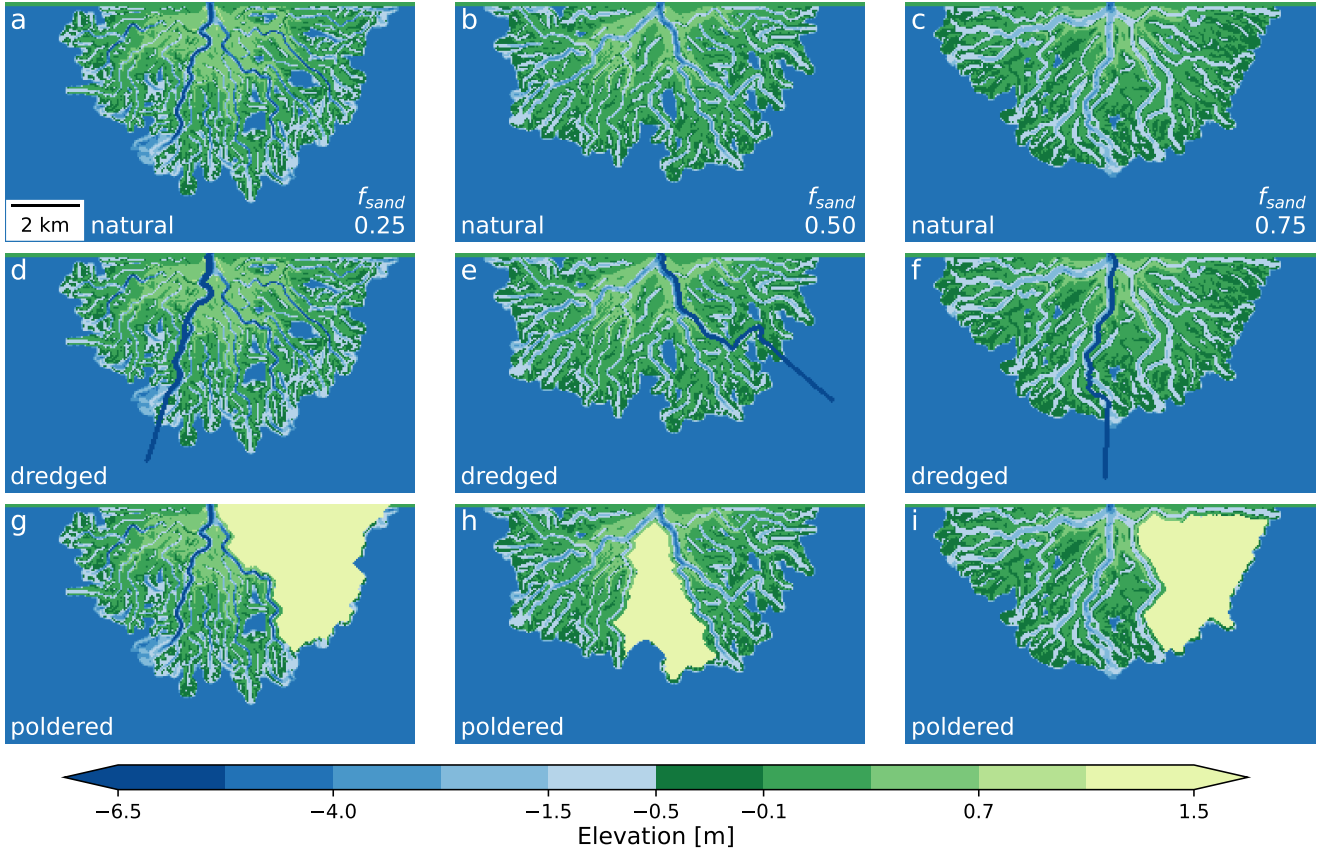
Figure 4. Examples of the different topography modifications. a, b, c: ‘‘Natural’’ delta topographies with no human modifications. d, e, f: ‘‘Dredged’’ delta topographies where the dominant channel has been dredged to a depth of 10 m below sea level. g, h, i: ‘‘Poldered’’ delta topographies where the largest island is identified and raised to an elevation of 10 m above sea level.
