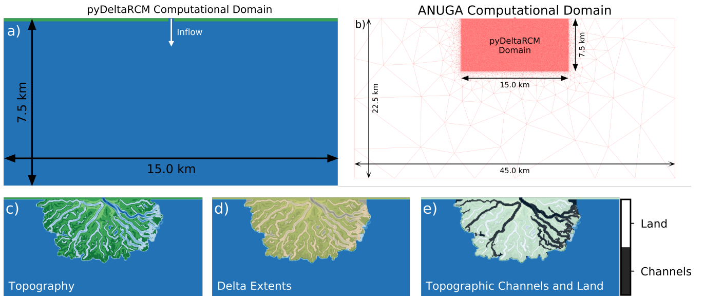
Figure 2. Examples a: The pyDeltaRCM computational domain. b: The ANUGA computational domain. c: An example of the two deltaic topography modification workflows starting from one final topography (a). b-e: d: The dredging workflow extracted delta extents for that topography. f-i: e: The poldering workflow extracted regions of channels and land, defined by topography, within the delta.
