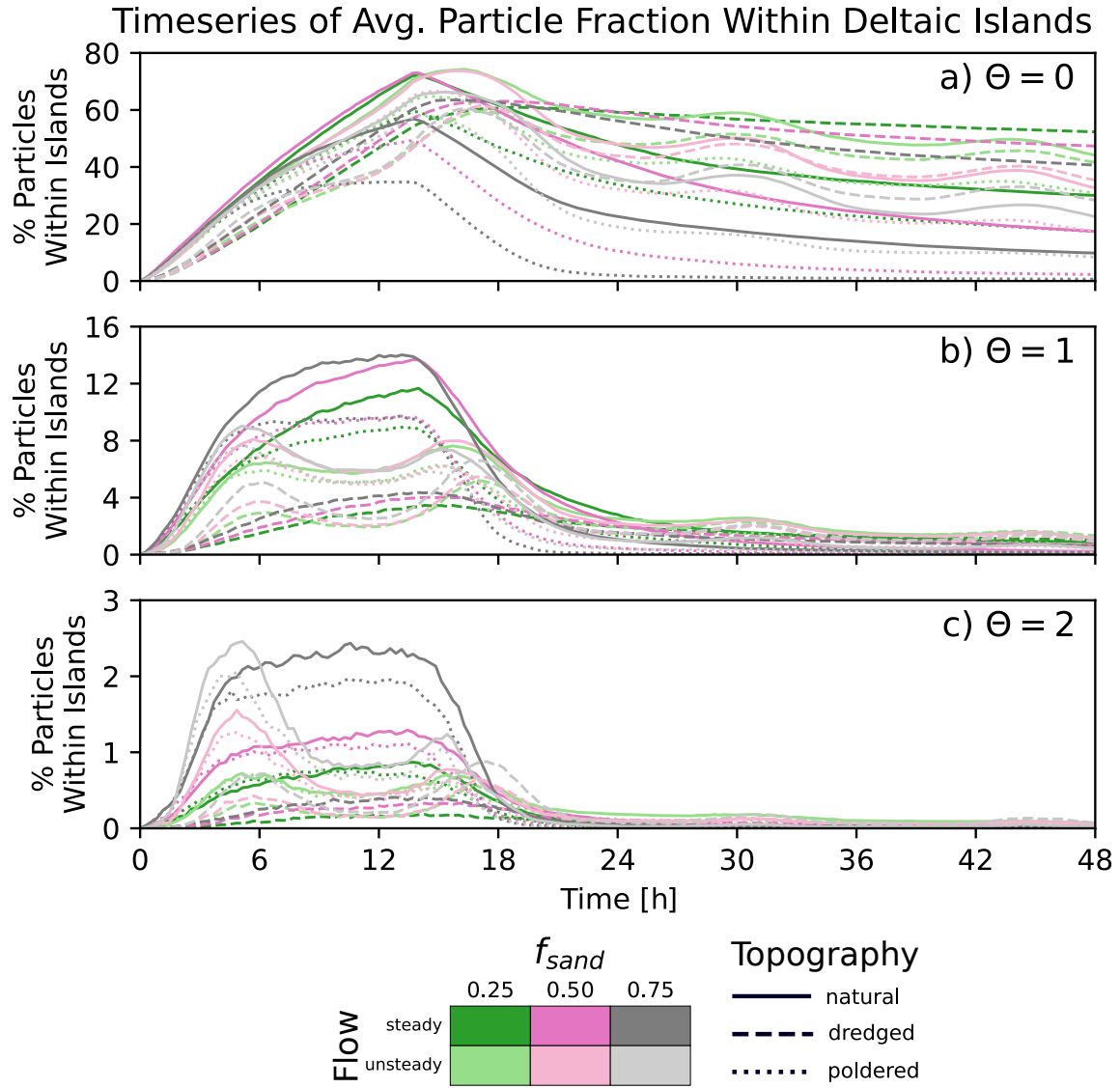
Figure 8. Timeseries of the average percentage of particles to be within deltaic islands for the first 48 hours over which the particles are routed for each modeled scenario. Data is grouped by \theta value, with a) \theta = 0 , b) \theta = 1 , and c) \theta = 2 . Note: Individual In all of the unsteady (tidal) scenarios (pale colors) the influence of the tidal signal is visible. For \theta = 1 and \theta = 2 the local maxima in the plots correspond to the flood tide peaks at hours 3 and 15. In a) , the natural topographies with 50% and 75% input sand fractions experience the highest fraction of particles visiting islands, while the poldered cases have the lowest values. In b) and c) higher input sand fractions correspond to higher fractions of particles entering islands, while the dredged topographies experience markedly low fractions of particles in islands across all time. Note that individual panels have different y-axis limits, in a) values near 80%, while in b) they only approach 15%, and in c) they only near 3%.
