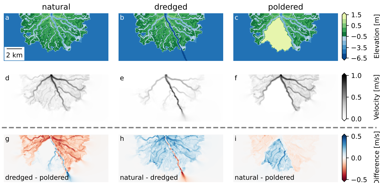
Figure 6. Visualizations of steady-state hydrodynamics (Section 2.3). a, b, c: Example model topographies. d, e, f: Corresponding ANUGA steady flow velocities. g, h, i: Difference maps between flow velocities from the scenarios shown in panels d, e, f .
