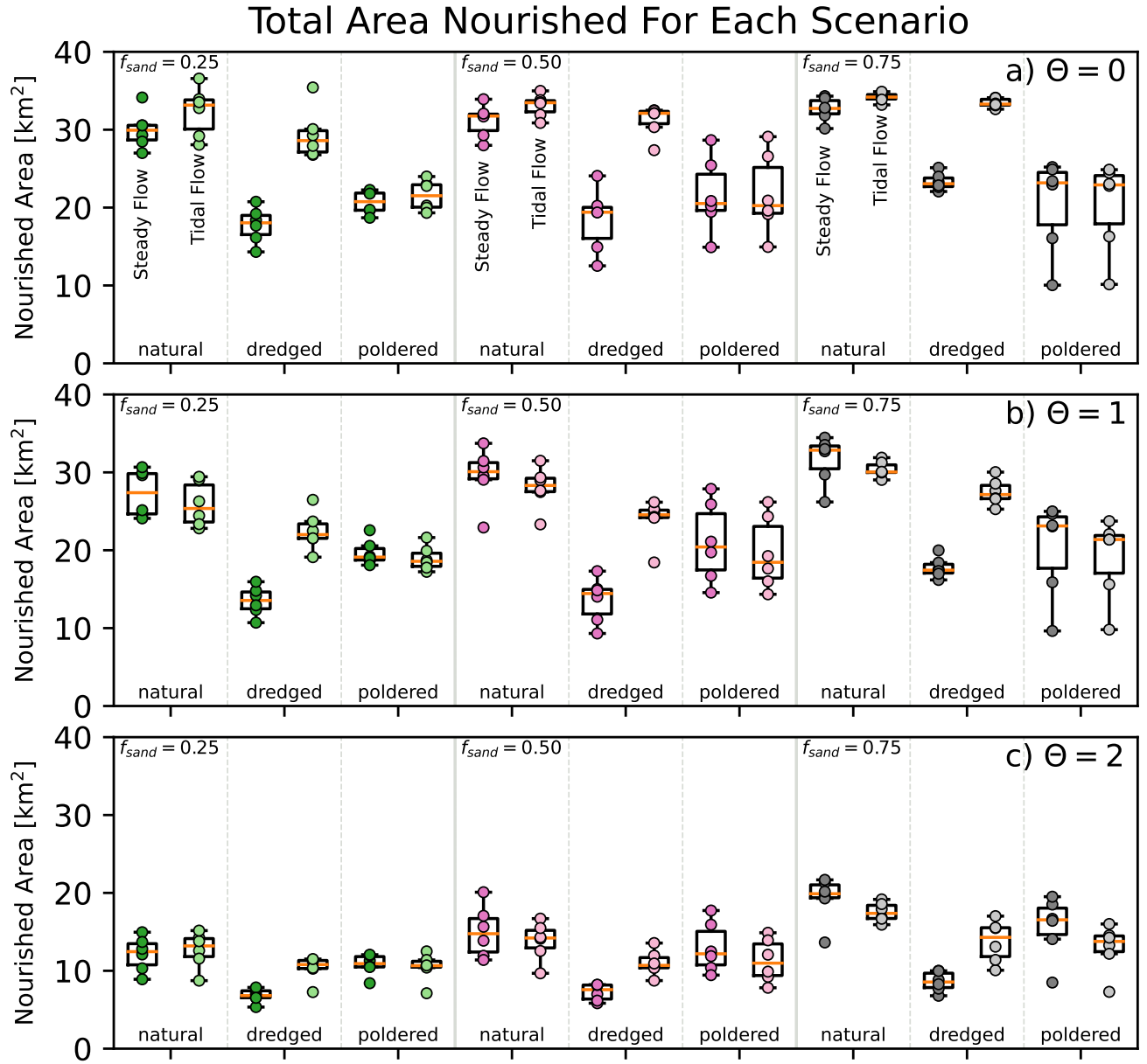
Figure 7. Total area nourished (visited) by particles for each scenario. Individual model replicate results shown as points overlaid on box-plots of the same data. Data are identified by input sand fraction, flow regime, and topographic modification, and further organized on separate axes by the \theta parameter with a) \theta = 0 , b) \theta = 1 , and c) \theta = 2 . For select individual particle paths see Fig. A5 & Fig. A6.
