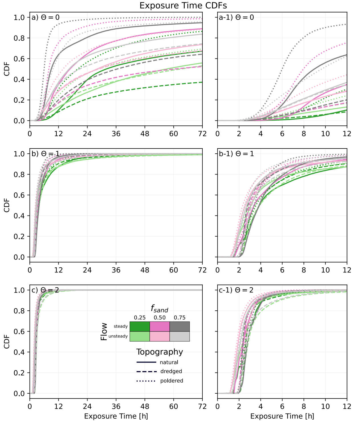
Figure 9. Exposure time cumulative distribution functions (CDFs) for the different scenarios calculated over the full delta extents (e.g., Figure 2d) . Data is grouped by \theta value, with a) \theta = 0 , b) \theta = 1 , and c) \theta = 2 , with the a-1 , b-1 , c-1 designations for zoomed in plots of the same data.
