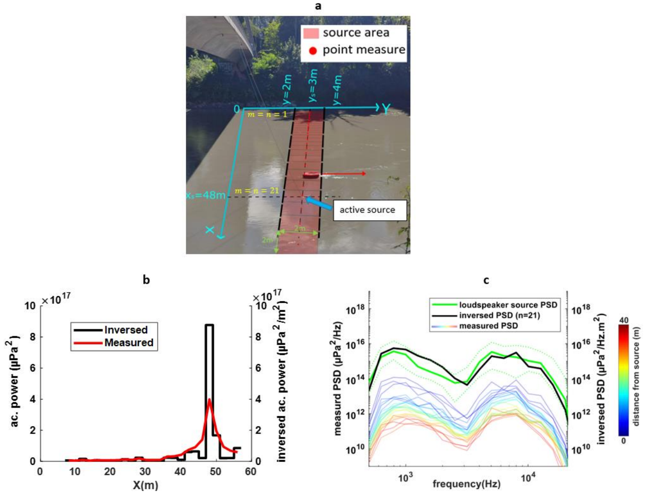
Figure 4 (a) Representation of the geometry of sources and acoustic measurements on the Iser River. (b) measured acoustic power P_{\varphi_n} ( \mu Pa^2 , red line) and the inversed source power P_{\hat{s}_m} ( \mu Pa^2 \cdot m^{-2} , black line). (c) measured spectrum at each position in the river \varphi_n ( \mu Pa^2 \cdot Hz^{-1} , faded color lines). The color index shows the distance of the measurement from the source which increases from blue to red. The inversed spectrum \hat{s}_m ( \mu Pa^2 \cdot Hz^{-1} \cdot m^{-2} , in black line) corresponds to the spectrum at location 47-49 m ( n=21 ). The green spectrum corresponds to the median of the lake measured spectrum with the dotted line corresponds to 5% and 95% percentiles.
