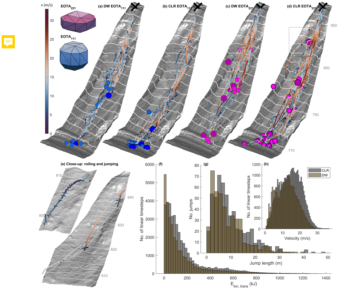
Figure 4. Velocities and deposition patterns of the 63 reconstructed rockfall trajectories: for the cubic EOTA_{111} rocks in (a) the forest state with deadwood (DW) and (b) the cleared forest state (CLR), and for platy EOTA_{221} rocks under (c) the DW and (d) the CLR site conditions. While the trajectories are color-coded according to the translational velocity, the same color coding as in Fig. 3 is used for the deposition points. The deposition pattern of the EOTA_{221} rocks stretches along the whole slope, compared to those of the EOTA_{111} rocks. The close-up views in (e) show the framed areas in (b) and (d). These enlarged displays feature a rolling trajectory (top) and a jumping trajectory (bottom). The rolling trajectory section visualizes the rock behavior after a tree impact. The succession of oblique jumps highlights the energy dissipation upon each rock–ground interaction with the subsequent accelerated airborne phase. The black crosses in (e) illustrate the identified contact points and their extent represents the uncertainty ranges for the impact locations. The uncertainties play a reduced role on the slope scale (a-d), as the crosses at every contact point are hardly noticeable any longer. The histograms highlight differences between the two forest states regarding (f) translational kinetic energy, (g) jump length, (h) and translational velocity.
