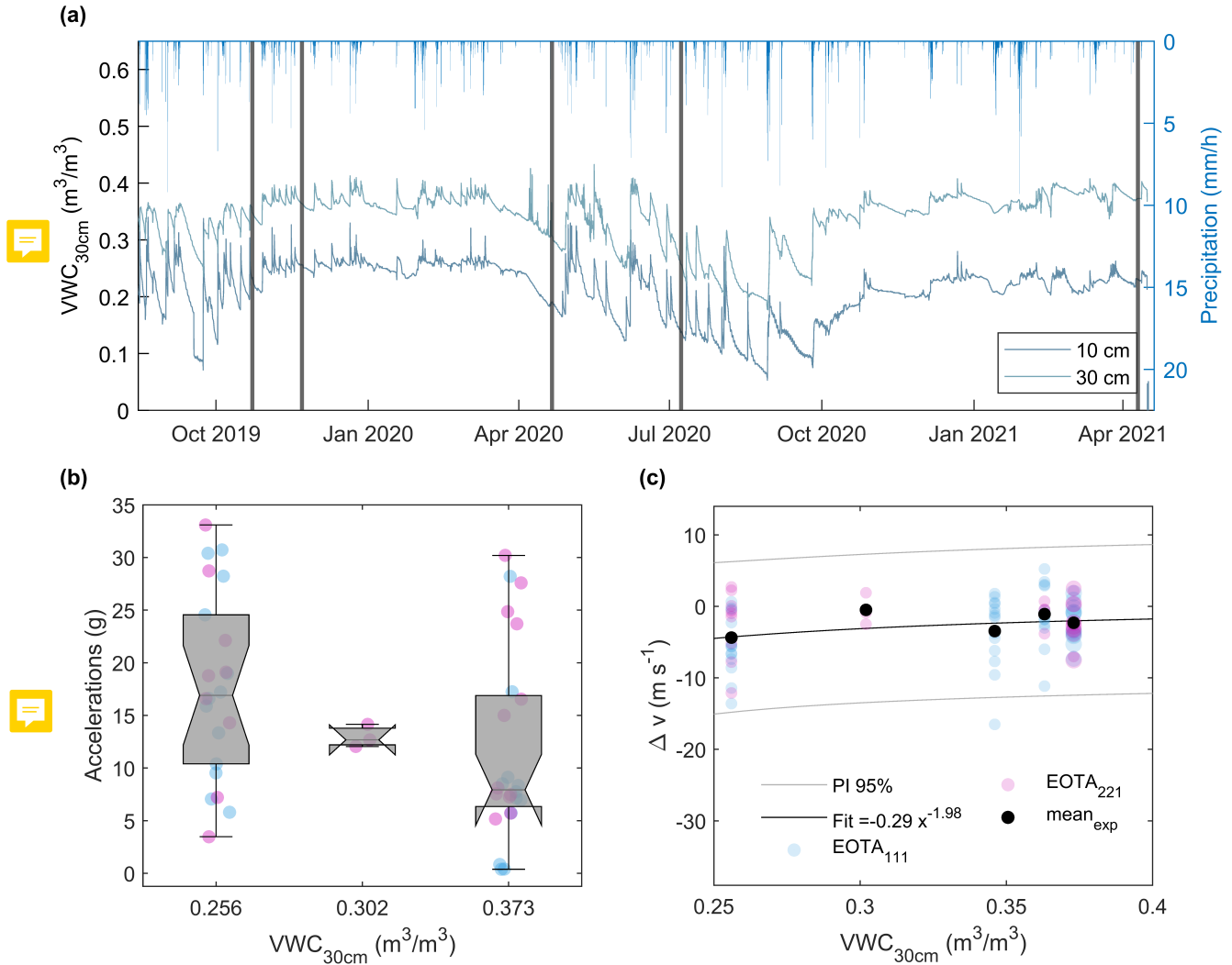
Figure 8. Soil moisture and its implications for rockfall impacts. (a) Volumetric water content (VWC) was measured at 10 and 30 cm depths over time compared with the precipitation measured at the closest MeteoSwiss weather station (4 km away, Federal Office of Meteorology and Climatology MeteoSwiss 2018). The vertical lines highlight the five experimental days with video coverage used for the trajectory reconstruction in Figure 4. (b) Accelerometer data versus VWC for soft soil impacts ( n = 49 ). The median values of the measured rock accelerations of all representative impacts within the region of the soil moisture sensors show a weak negative correlation with the measured VWC. (c) Velocity changes \Delta v related to the observed VWC, with rock mass represented by symbol size ( n = 78 ). The prediction interval (PI) is \pm 10.6 \text{ m s}^{-1} .
