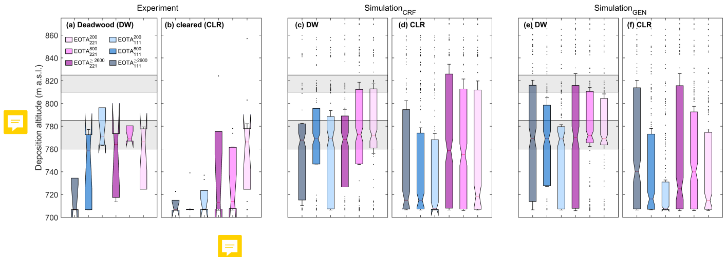
Figure 10. Summary boxplots of the deposition altitudes for deadwood (DW) and cleared (CLR) forest states, expressed as elevation in m a.s.l. (a) Experiment DW, (b) experiment CLR, (c) close-to-reality (CRF) simulation DW (d) CRF simulation CLR, (e) simulation with generic forest setup and DW, and (f) GEN simulation CLR. The shaded areas depict the elevations of the two deadwood clusters, with the lower, main deadwood cluster spanning 785–760 m a.s.l. The boxplots feature the median values, with standard box sizes of one interquartile range (IQR), comprising 50% of all values. The boxes are colored according to their weight and shape classifications. The whisker length is compared with standard boxplots reduced to 0.1·IQR.
