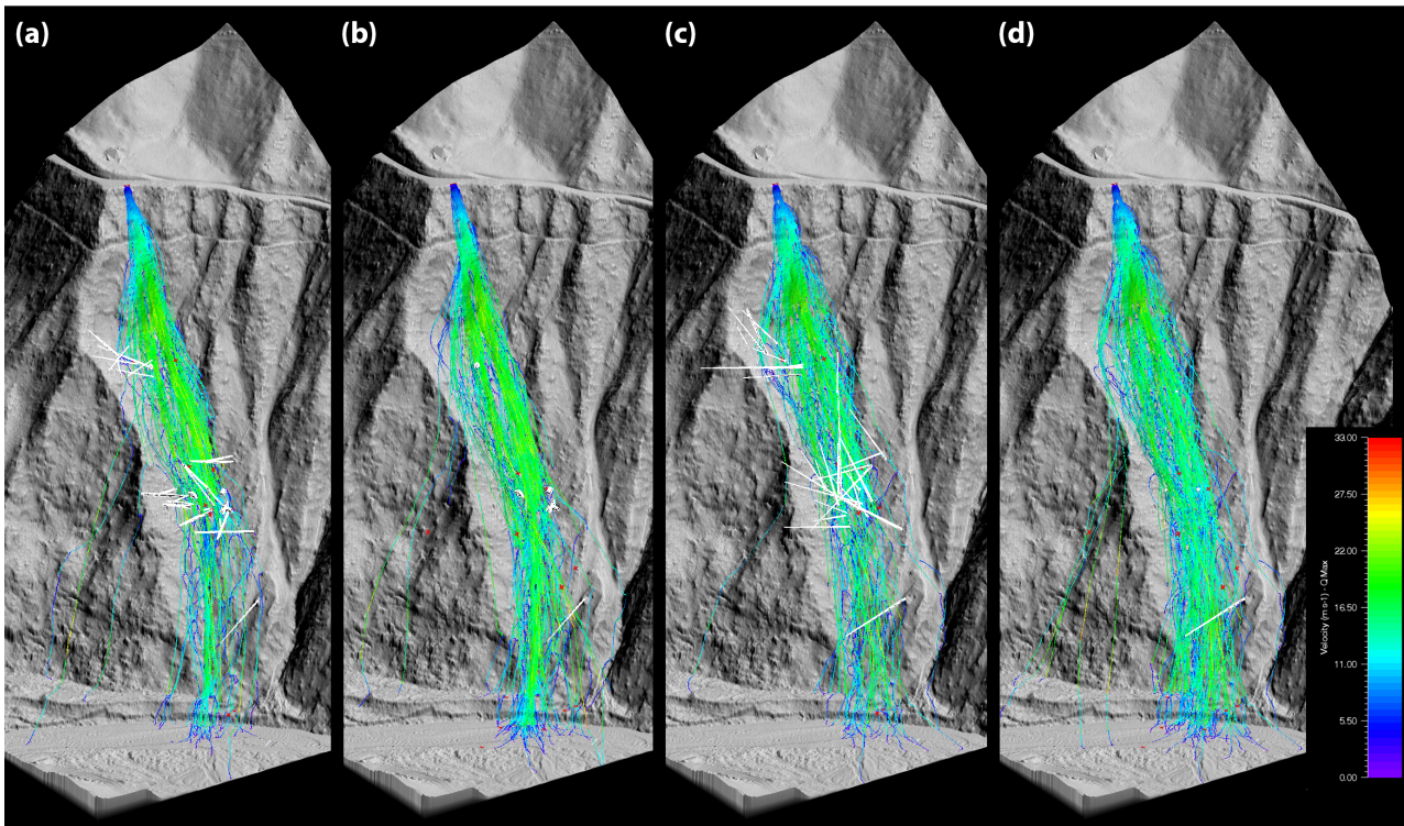
Figure 9. Visualization of the RAMMS::ROCKFALL simulations for EOTA _{221}^{800 \text{ kg}} . (a) and (b) Close-to-reality (CRF) setup, with forest information extracted via commercial TerraScan software from a high-resolution lidar point cloud complemented with on-site, manually measured and digitized deadwood (white lines), for (a) the deadwood (DW) scenario and (b) the cleared forest (CLR) scenario, which served as a calibration scenario. (c) and (d) Generic scenario with standing trees randomly generated within RAMMS::ROCKFALL, based on estimates of the number of trees per hectare, the mean DBH, and its standard deviation, for (c) the DW scenario and (d) the CLR scenario. The deadwood in (c) originates from the automatic deadwood generator (Ringebach et al., 2022a).
