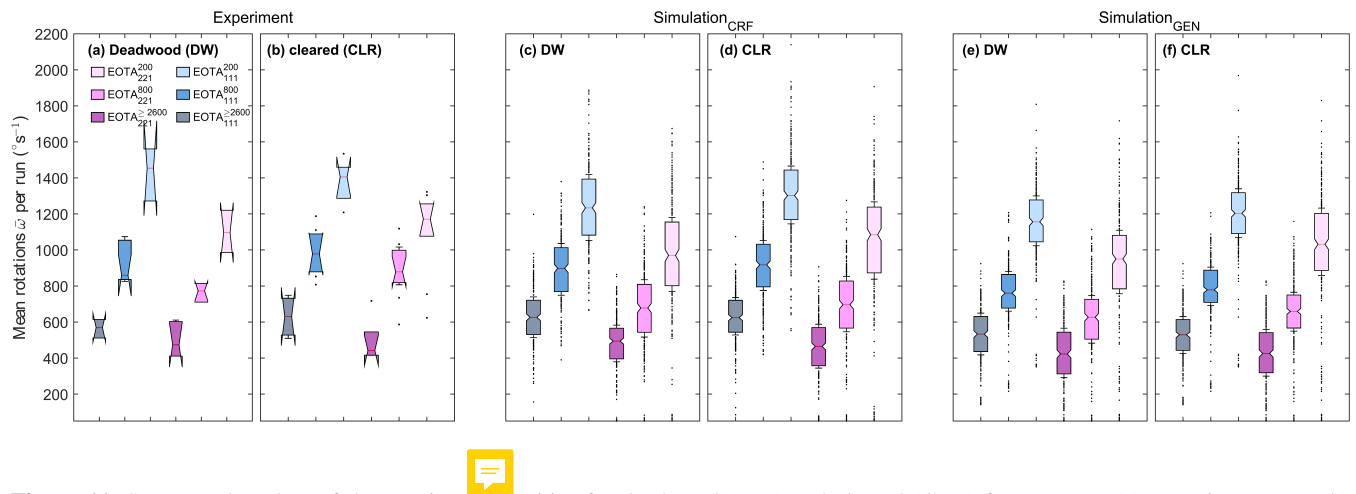
Figure 11. Summary boxplots of the rotational velocities for deadwood (DW) and cleared (CLR) forest states. (a) Experiment DW, (b) experiment CLR, (c) close-to-reality (CRF) simulation with DW, (d) CRF CLR, (e) generic forest setup (GEN) DW, and (f) GEN CLR. The boxplots feature the median values, with standard box sizes of one interquartile range (IQR). The boxes are colored according to their weight and shape class classifications, and whisker length = 0.1·IQR.
