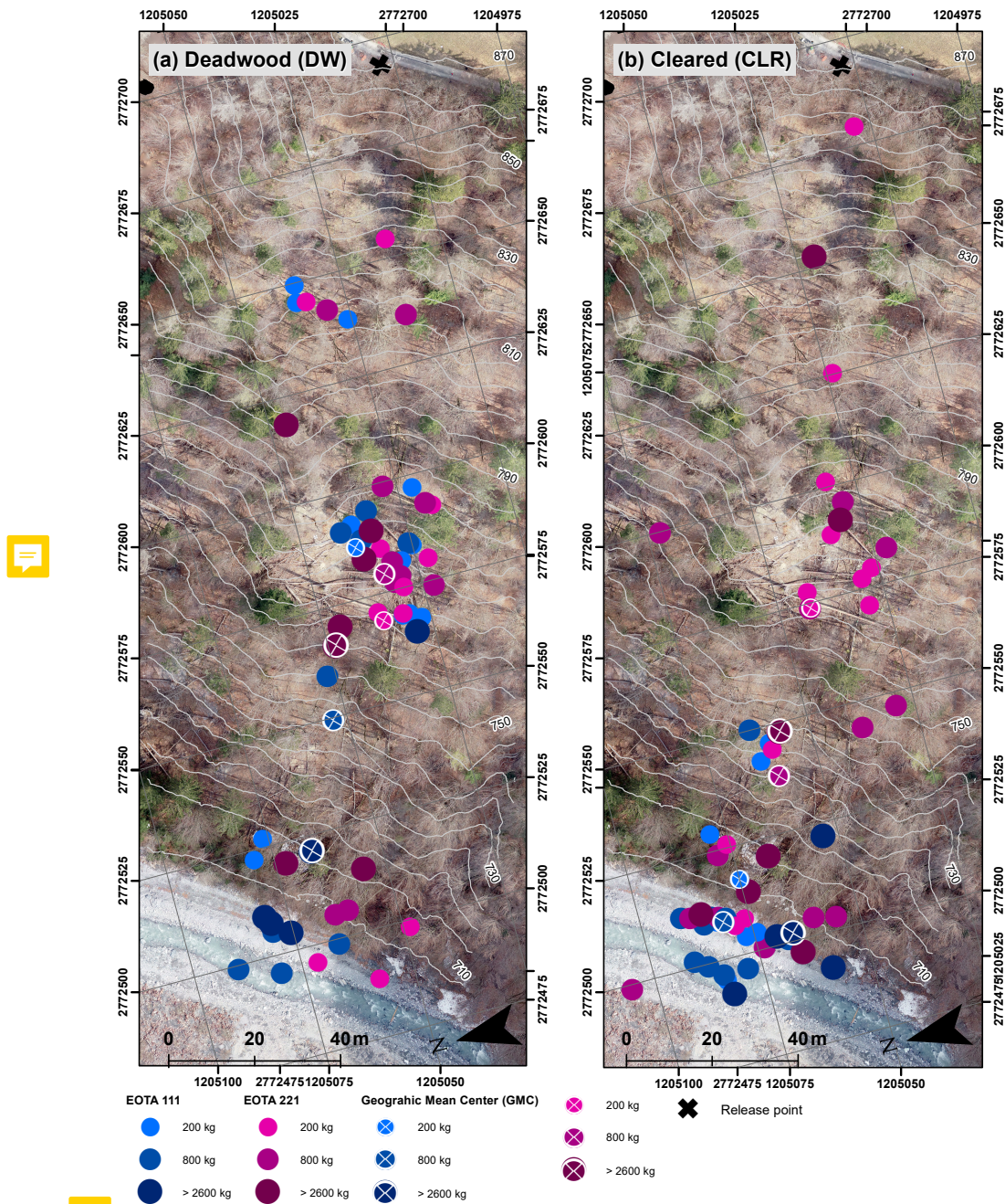
Figure 3. Complete deposition patterns of all 106 rocks for the two different forest states (a) with lying deadwood logs and (b) after clearing of the deadwood logs. Blue markers represent the deposition points of cubic EOTA 111 rocks varying from 200 kg (light blue) to > 2600 kg (dark blue). Magenta markers represent the deposition points of platy EOTA 221 rocks varying from 200 kg (light magenta) to >2600 kg (dark magenta). The respective geographic mean centers for each rock category are indicated with a circle in the same color but marked with a cross.
