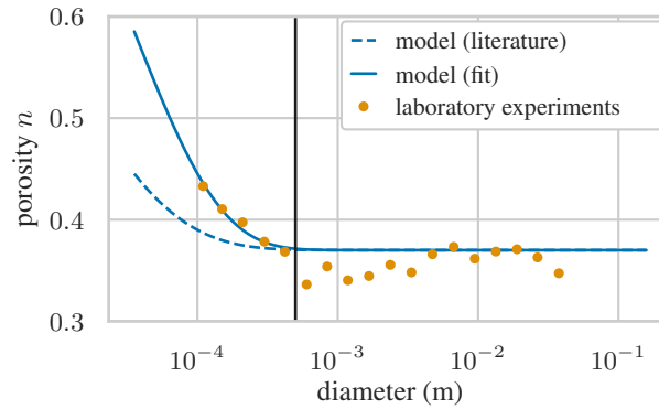
Figure 10. Effect of cohesion on porosity of uniform packings of a given mean diameter. Data from laboratory experiments with sediment from the Rhine River (Frings et al., 2011), corrected for edge effects of the used container for the measurements. The solid black vertical line denotes the assumed d_c^{coh} of 0.5 mm.
