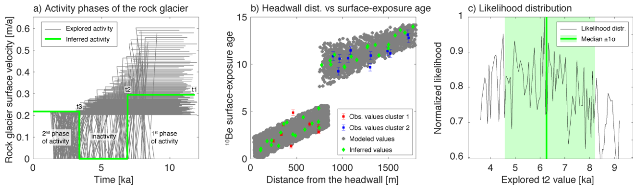
Figure 11: a) Activity phases of the rock glacier defined as the evolution of the rock glacier surface velocity in time (explored histories and best-fitting history are shown respectively, grey and green lines). b) Relationship between 10 Be surface-exposure age and distance to the headwall. Observed values of the cluster 1 and 2, respectively, in red and blue squares. Modelled and best-fitting values in grey and green respectively. c) Likelihood distribution of the inversion exploring the time at which the 1st phase of activity ends (t 2 ). See text for details.
