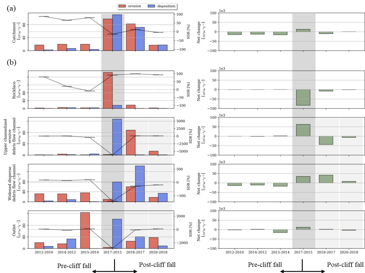
405 Figure 6. Time series of geomorphic sediment budgets. a) Geomorphic sediment budgets at the catchment scale. b) segregated sediment budget into the four morphodynamic zones. Left column: The bar plot depicts yearly volumes of erosion in red and deposition in blue (units at the left axis). The black line indicates the sediment delivery ratio expressed as the proportion of sediment leaving the morphodynamic zone from the total net erosion (units at the right axis). Right column: yearly net change calculated as the difference between erosion and deposition. The estimated uncertainty of the absolute volume is less than 2% thus, imperceptible due to the scale of the graph. Dark grey polygons highlight the temporal stamp at which the cliffs fall took place. Lighter grey indicates the system response two and four years after the event. Note how the reverse net changes propagate downslope the system thought time.
