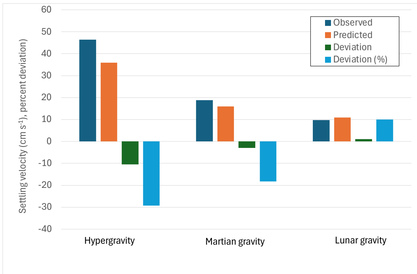
Figure 8: Comparison of observed and predicted settling velocities based on the maximum difference between the predicted and observed terminal settling velocities at the three gravities. The deviation ( \text{=predicted} - \text{observed} ) is negative for Martian and hypergravity, indicating an underestimate of the predicted terminal velocities, while is slightly positive at lunar gravity, where the observed settling velocity is lower with respect to the predicted by the Ferguson and Church model.
