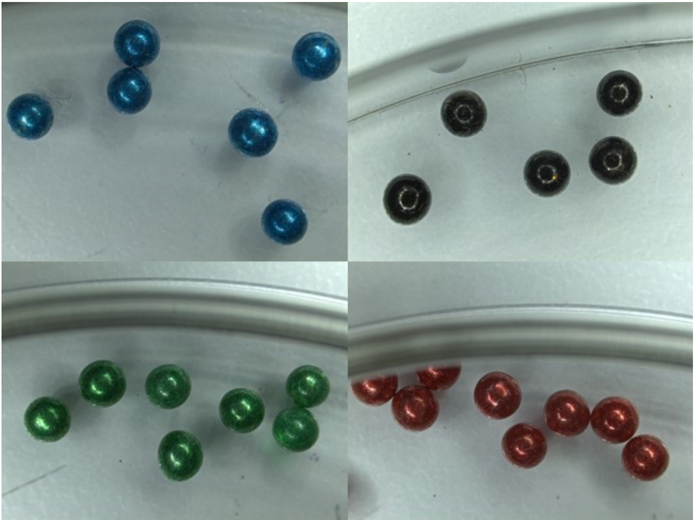
Figure 5: Glass spheres used for CompSedMars I. The particles are all spherical, a diameter comprised between 1.7 and 2.0 mm, and have four distinct colours to be better distinguished in the particle tracking software. Image credit B. Kuhn.
