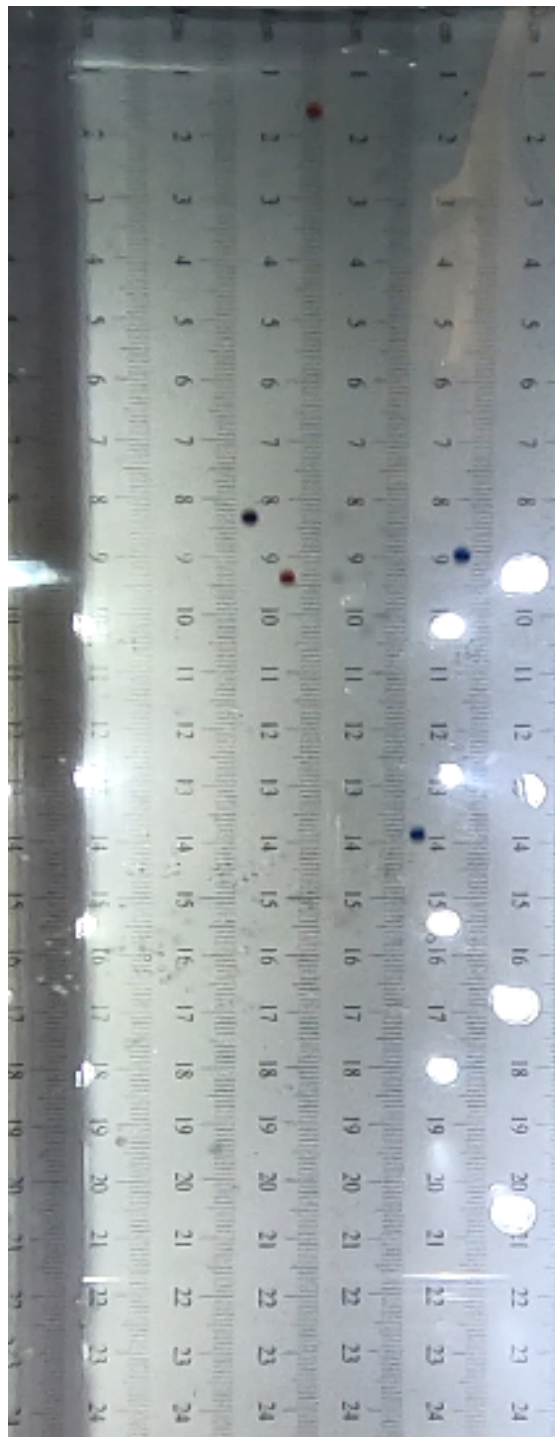
Figure 6: Snapshot captured from a video produced by one of six Go Pros used to record the trajectories of free-falling particles in liquid water at Earth gravity conditions. Five glass reference spheres are observed. The graduated scale in the background was used as a reference to extrapolate the position of the particles as a function of time. In this picture, the lack of distortion by using the linear field of view mode of the GoPro can be seen.
