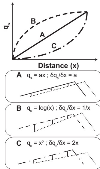
Figure 9. Schematic of different patterns of erosion along the stoss side of a bedform based on linear (A), logarithmic (B), and exponential algebraic (C) increases in bedload transport.
