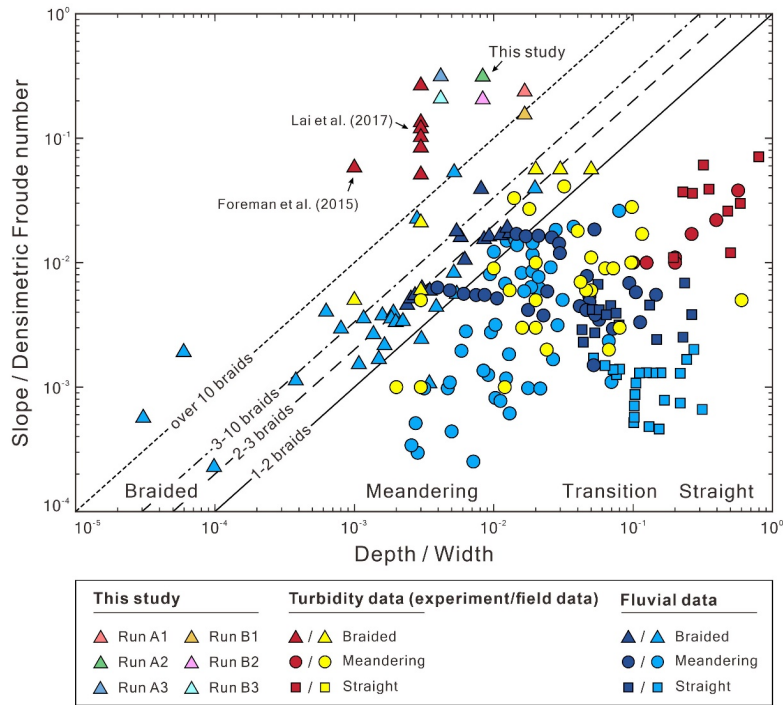
Figure 14. Morphological classification of fluvial rivers and submarine channels (modified after from Parker, 1976 and Lai et al., 2017).
