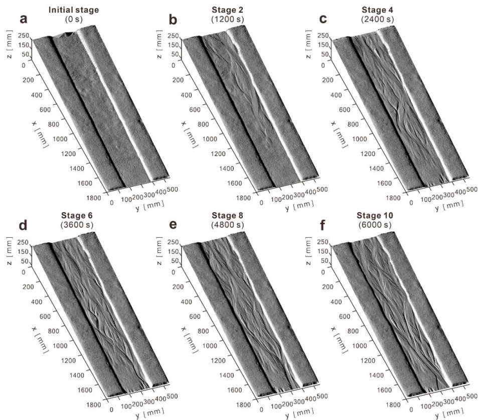
Figure 5. Hillshaded-DEMs-DEM hillshades for Run A2 from t = 0 to 400-6000 mins.
