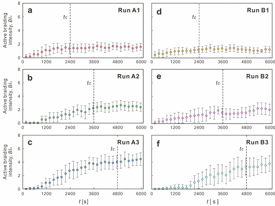
235 Figure 7. Evolution of active braiding intensity ( BI_A ) for (a)-(c) Runs A1, A2 and A3; (d)-(f) Runs B1, B2 and B3; t_c is the critical time for BI_A reaching a stable phase, each run.
