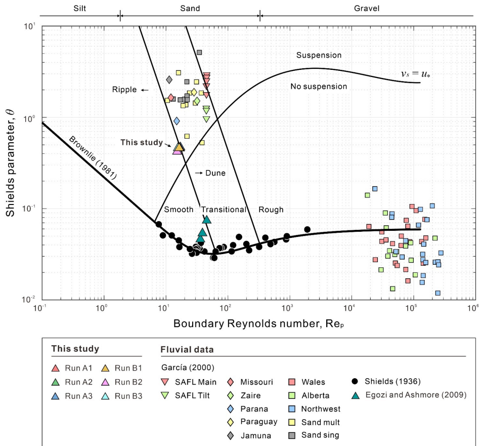
Figure 15. Shields diagram of fluvial rivers and submarine channels (modified after García, 2000).
