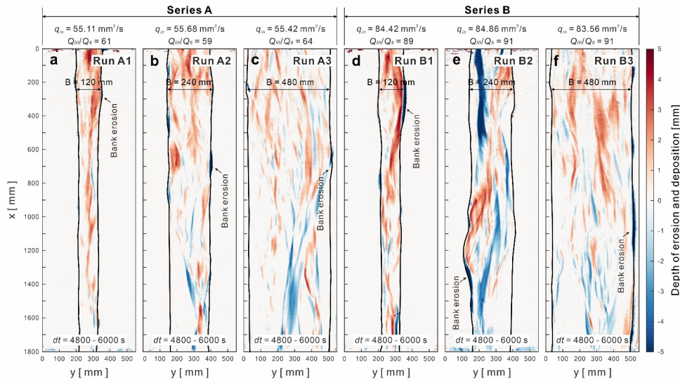
Figure 8. The DEM of difference (DoDs) for Series A ( q_{in} \approx 55 \text{ mm}^2/\text{s} , Q_{in}/Q_s \approx 60 ) and Series B ( q_{in} \approx 84 \text{ mm}^2/\text{s} , Q_{in}/Q_s \approx 90 ). The time duration for DoD calculation is dt = 4800\text{-}6000 \text{ s} (last 20 min).
