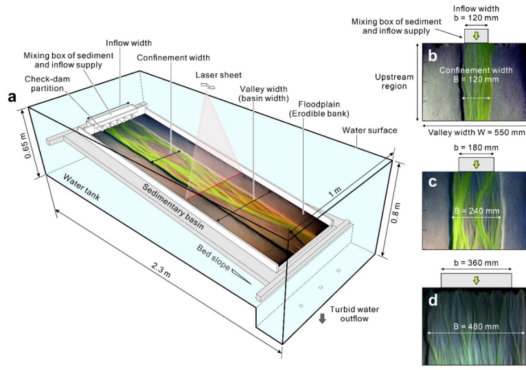
Figure 2. (a) Experimental setup for studying the evolution of submarine braided channels with different confinement widths and inflow-to-sediment discharge ratios; (b) inflow width, confinement width and valley width of Runs A1 and B1; (c) inflow width, confinement width and valley width of Runs A2 and B2; (d) inflow width, confinement width and valley width of Runs A3 and B3.
