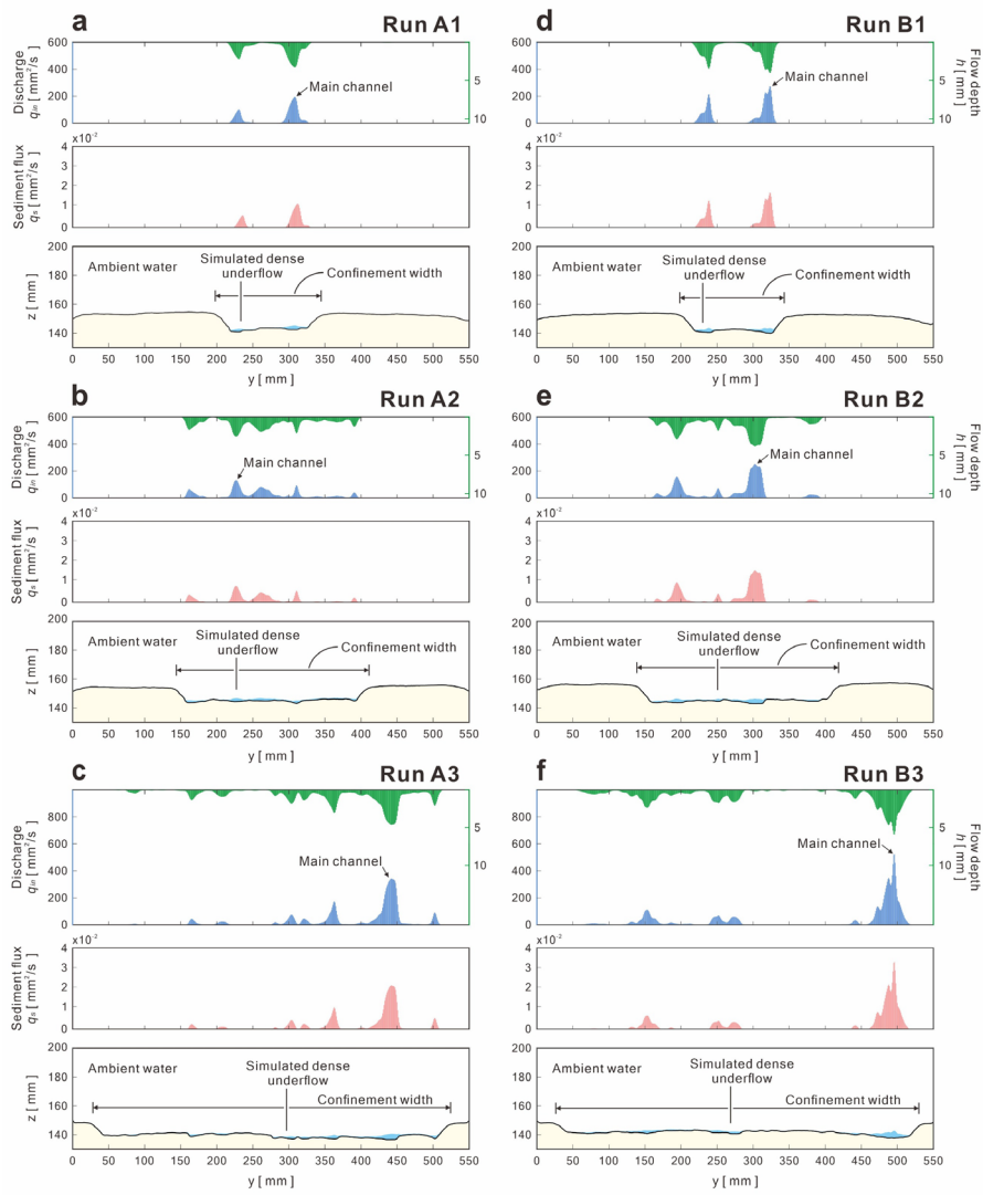
[295] Figure 11. Simulated discharge, flow depth and sediment flux extracted at the midstream ( x = 900-1000 mm) for each run.
